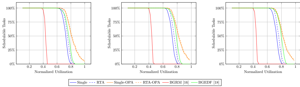
(a) 2-1 (b) 3-1 (c) 4-1
