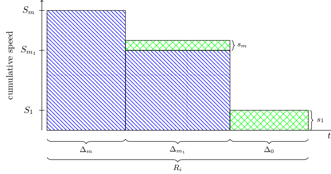
■ Figure 4 Execution of higher-priority jobs hp(i) (blue diagonal lines) and job J_i ( i > m ) under analysis (green cross-hatching) upon a two-speed multiprocessor (with m_1 fastest processors).
