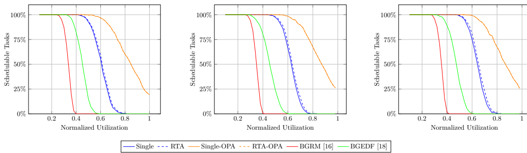
(a) 2-2-1-1 (b) 3-2-2-1 (c) 4-3-2-1
