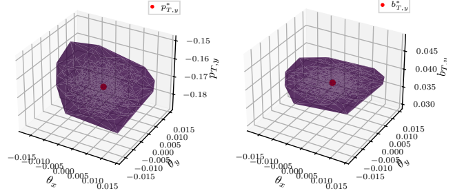
Fig. 2: Solution space example of p_{T,y} (left) and b_{T,y} (right) as a function of the DCM disturbance \boldsymbol{\theta} \sim \mathcal{N}(0, 0.005) generated with 1000 samples. The optimal solution is represented in red, and no inequality constraints is active.
