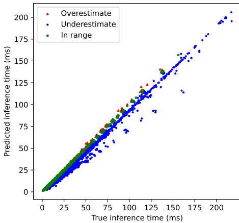
Fig 4. Evaluation results on the test dataset. Green, blue, and red dots represent instances with |Deviation| < 1 ms, Deviation < -1 ms, and Deviation > 1 ms, respectively.
