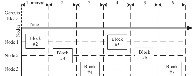
Fig. 3: Block creation in PoA Consensus Algorithm
