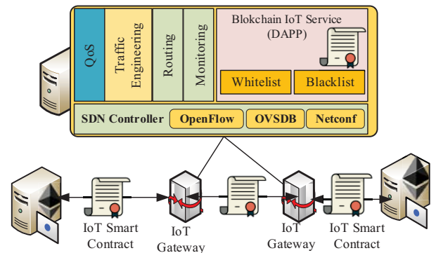
Fig. 5: Ensuring Security and Interoperability between IoT Gateways.
