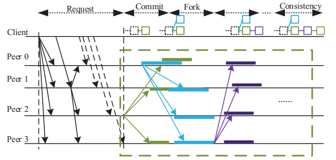
Fig. 8: Message Exchange in lottery-based PoET
