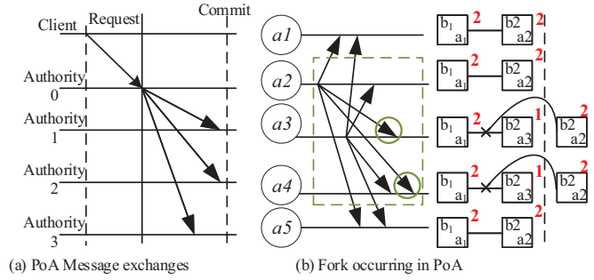
Fig. 6: Message Exchange in PoA
