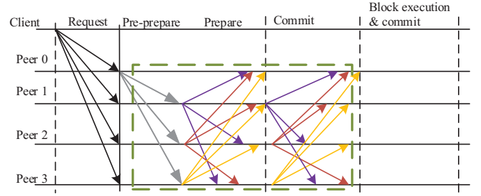
Fig. 7: Message Exchange in voting-based PBFT
