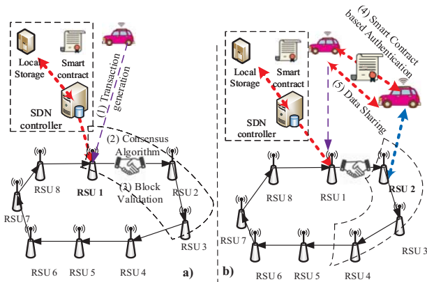
Fig. 4: Secure message dissemination in SDN-enabled VANET
