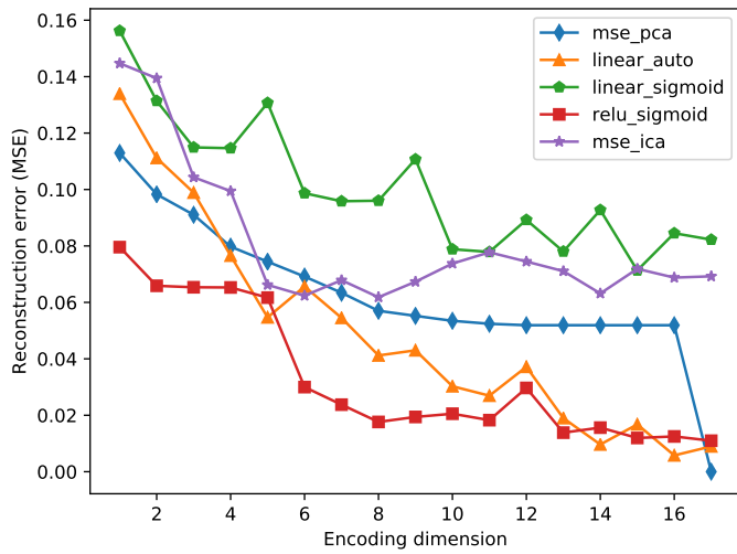
Fig. 3: Data Pre-Processing
