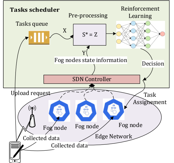
Fig. 1: Task Scheduling architecture
