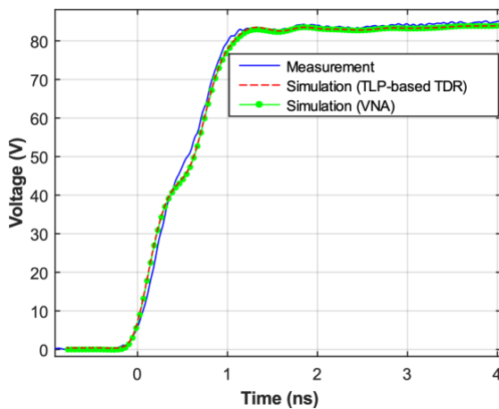
Fig. 7. Transient measurement vs simulations using VNA and TLP-based TDR models for 470 \Omega load
