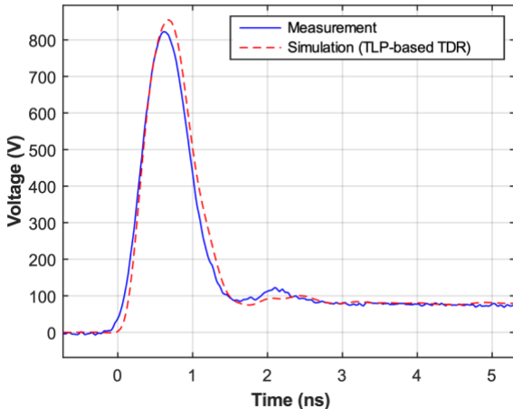
Fig. 15. Transient measurement vs simulation of TVS2 for 2 KV TLP pulse
