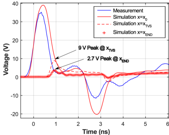
Fig. 18. Transient measurement and simulation of a 80 V HMM pulse TVS1+CRC network.
