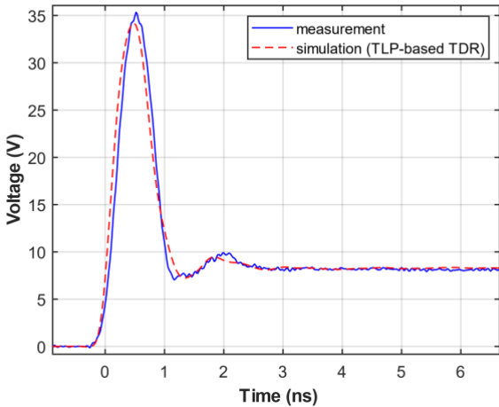
Fig. 14. Transient measurement vs simulation of TVS for 80 V TLP pulse
