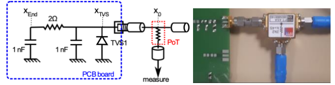
Fig. 16. Schematic and picture of the CRC+TVS network
