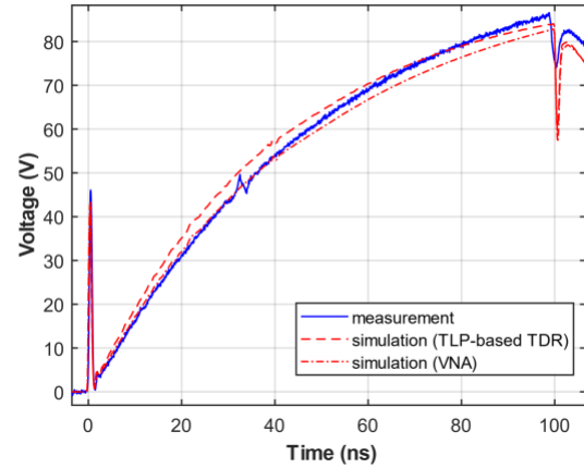
Fig. 8. Transient measurement vs simulation for COG capacitor load
