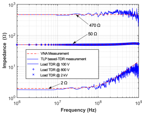
Fig. 4: Comparison of the impedance obtained by TLP-based method and VNA for 2 \Omega , 470 \Omega load and calibration on 50 \Omega load
