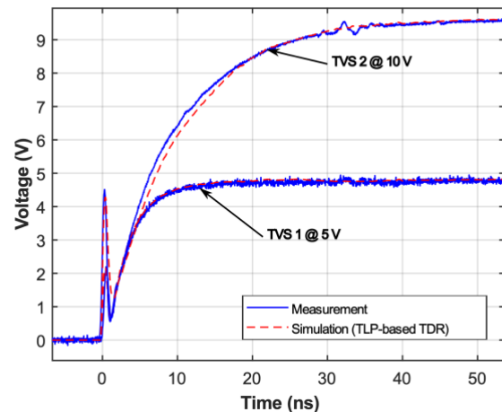
Fig. 13. Transient measurement vs simulation of TVS for 5 V TLP pulse
