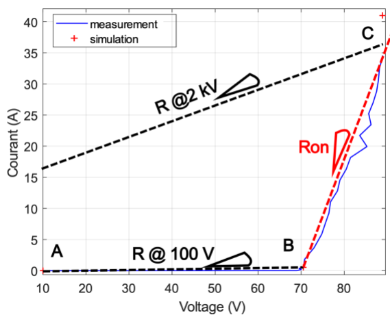
Fig. 11. Quasi-static I(V) curve of the TVS2.
