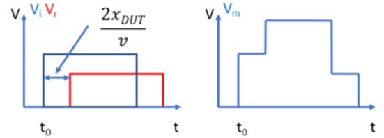
Fig. 2. Example of TDR waveform for an unmatched load
