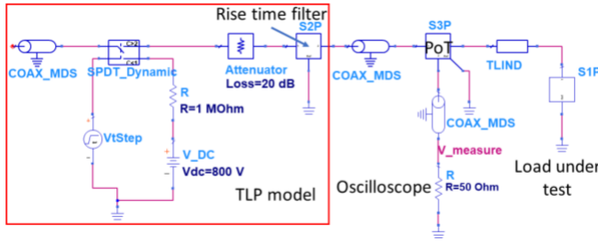
Fig. 6. Electrical diagram simulation into ADS software.
