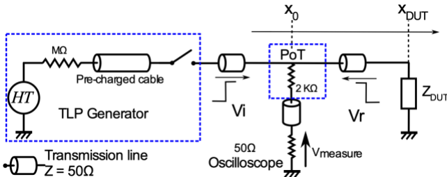
Fig. 1. Principle of the TLP-based TDR measurement method
