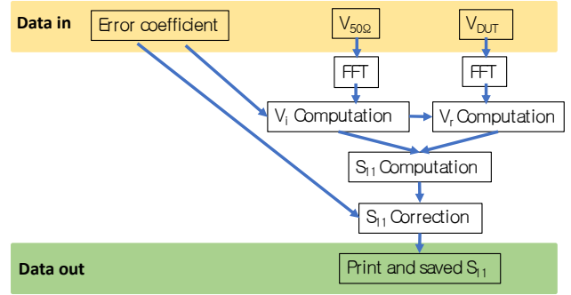
Fig. 3. Flow diagram of the model extraction method
