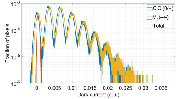
Fig. 8. Simulated dark current distributions at 67 °C for a 1-megapixel image sensor containing V_2 ( -/- ) and C_iO_i ( 0/+ ) defects, with \lambda of 5 and 2, respectively. Trap parameters are taken from [4]: (E_T, \sigma_n) = (-0.23 eV, 4.0 \times 10^{-15} cm ^2 ) and (-0.36 eV, 1.9 \times 10^{-15} cm ^2 ), respectively.
