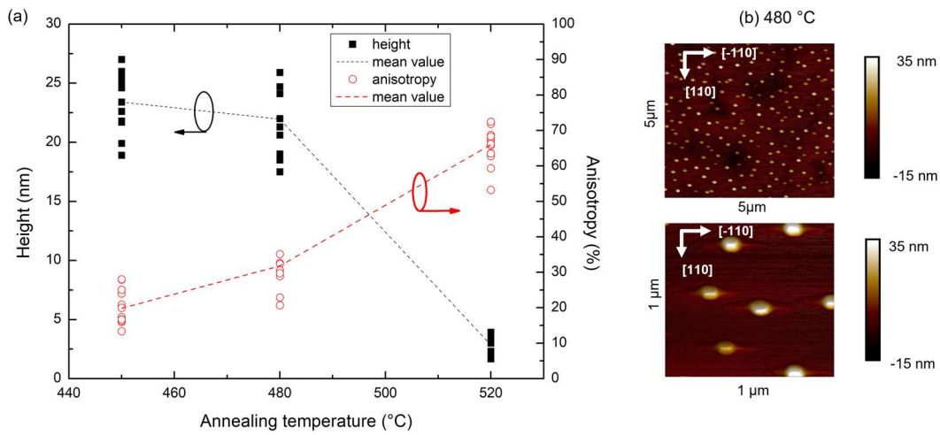
Fig.1. (a) Measurement of the height (solid black squares) and anisotropy factor (open red circles) of the GaAs QDHs as a function of the annealing temperature (measured at 5 positions on the 2-inch wafer/ dotted line: average values). (b) AFM images of the selected QDHs (480 °C, height: 21.94 nm, length: 141.94 nm, width: 101.97 nm, anisotropy: 28 %) acquired on 5x5 \mu\text{m}^2 (top) and 1x1 \mu\text{m}^2 (bottom) surfaces. (Note that AFM measurements were also taken at 45° to the direction of these images to check the absence of artifact).
