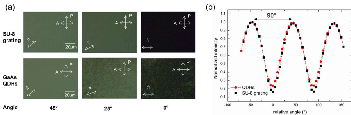
Fig. 3. (a) Images of the cells' surface observed with an optical microscope (reflection mode, X20, white light illumination) between crossed polarizers for 3 different angles between the LC director and the analyser axis ( 45^\circ , 25^\circ and 0^\circ ): (top) SU-8 \mu -cell, (bottom) QDHs \mu -cell. (b) Normalized reflected light measured as a function of the angle for the SU-8 grating \mu -cell (black squares) and for the QDHs \mu -cell (red circles) (reflection mode, X20, white light filtered with a 696 nm narrow band optical filter).
