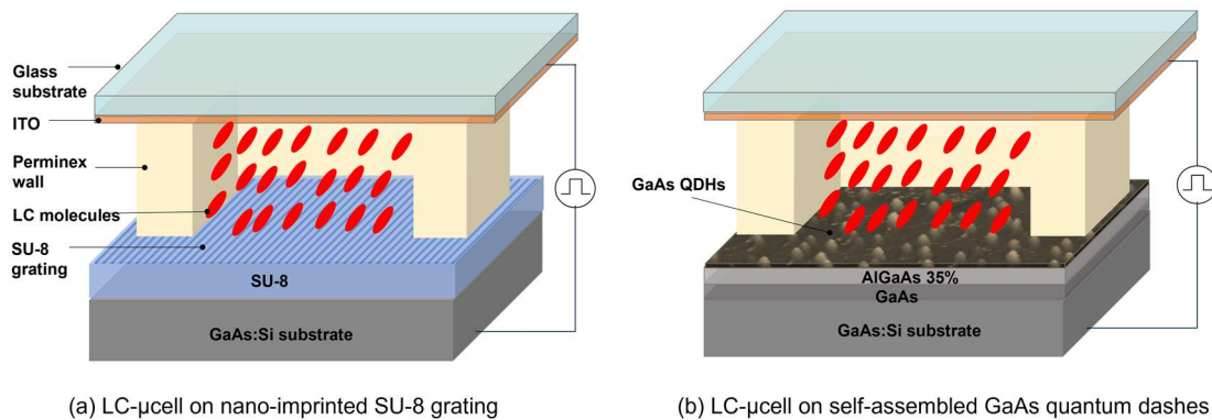
Fig. 2. Schematic cross view of LC \mu -cells fabricated on a N-doped GaAs substrate: (a) with a reference SU-8 nanograting (period: 200 nm/ groove depth: 48 nm/ duty cycle: 50 %, SU-8 layer; 700 nm) (b) with GaAs QDHs (height \sim 22 \text{ nm} , anisotropy \sim 28 \% , density: \sim 7 \text{ QDHs}/\mu\text{m}^2 ). The area of each \mu -cell is 2,8 \times 2,8 \text{ mm}^2 .
