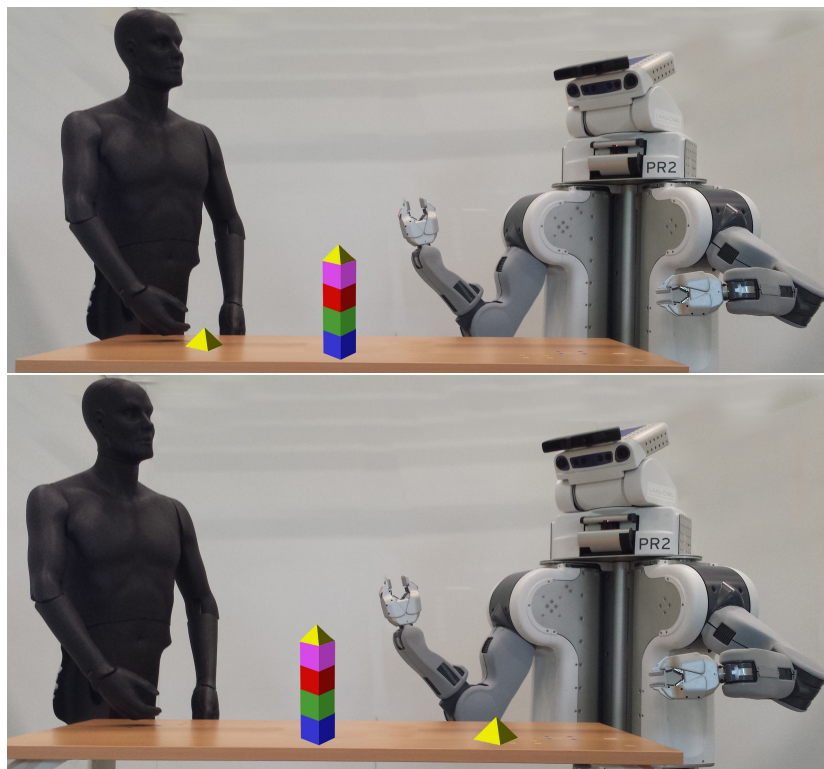
Fig. 2 Possible final states.
