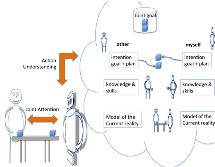
Fig. 3 Knowledge and processes for joint action. The robot builds and maintains a distinct mental model of itself and of its human partner concerning the state of the world. It also reasons and builds its own behaviour based on its estimation of its human partner intentions, knowledge and skills.
