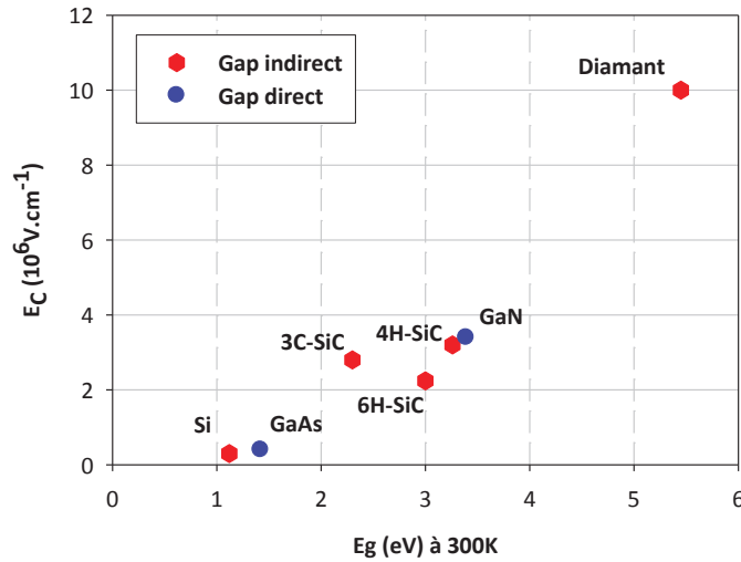
FIGURE 1.5 – Critical breakdown fields for different semiconducting materials with a doping concentration of 10^{16} \text{ cm}^{-3} depending on their gap (at 300 K)[8]
