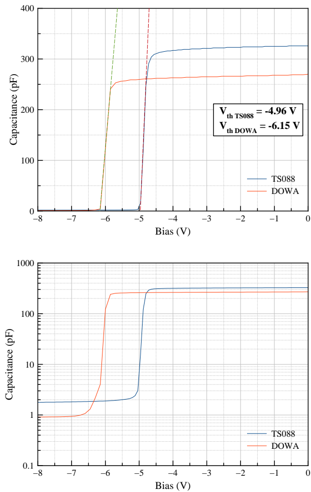
FIGURE 4.18 – Linear (up) and logarithmic (down) C(V) response for a PEALD MIS 400\ \mu\text{m} diameter diode during accumulation for samples from a DOWA and III-V Lab wafers. The \text{Al}_2\text{O}_3 thickness is 10 nm and the sampling frequency is 100 kHz for both samples.
