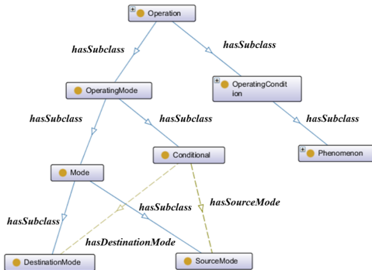
Figure 1.7: Operation Ontology
