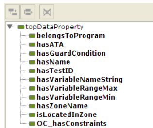
Figure 1.5: Data Properties
