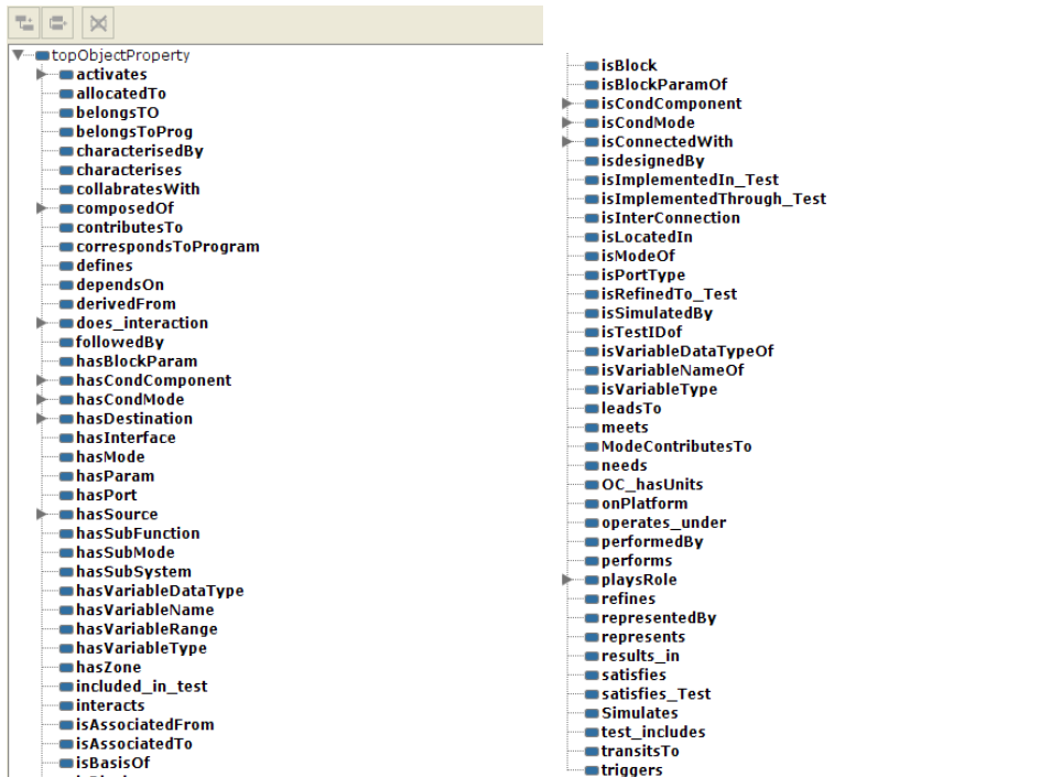
Figure 1.4: Object Properties
