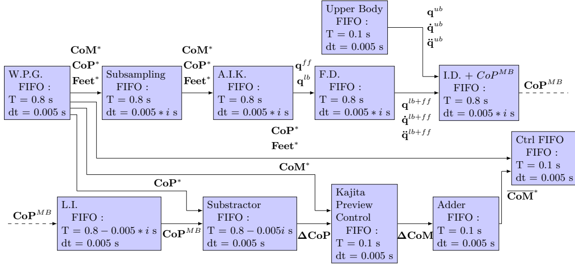
Figure A.1: This scheme describe the action of the dynamic filter. It contains all needed information in order to filter a desired CoM trajectory ( \mathbf{CoM}^* ) knowing the associated feet and CoP trajectories ( \mathbf{Feet}^* , \mathbf{CoP}^* ). See Subsec. A.1.2 for all the details.
