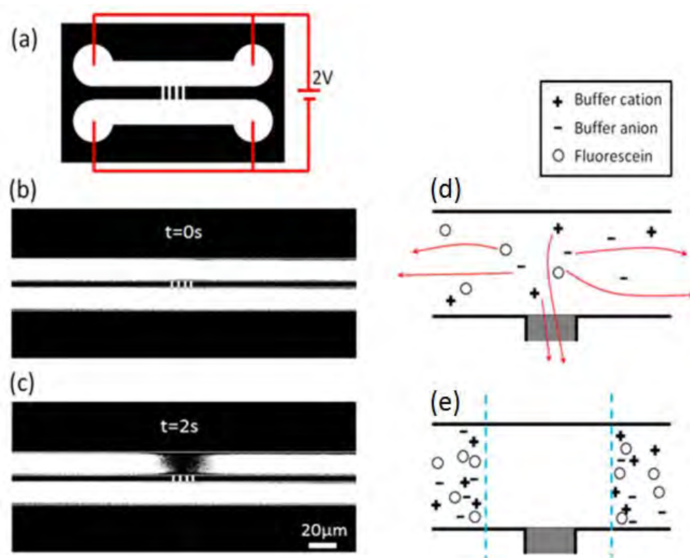
Figure 12. Ion depletion zone is formed at the anodic microchannel when 2 V is applied across PSi membrane using fluorescein 1\mu M in PBS 0.1 \times (pH 7.4). (a) Electrical connections. Optical pictures and schematics of the fluidic chip upon application (b, d) and 2 s after applying (c, e) 2 V across the membrane.
