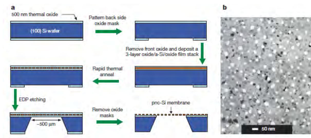
Figure 18. Fabrication and pore morphology of porous nanocrystalline (pnc) silicon membrane [16]. (a) Standard microfabrication tools are used to deposit, pattern and suspend pnc-Si films. (b) A plan-view TEM image of the porous nanostructure of a 15-nm-thick membrane. In this bright field image, pores appear as bright spots while nanocrystalline silicon is in grey or black contrast.
