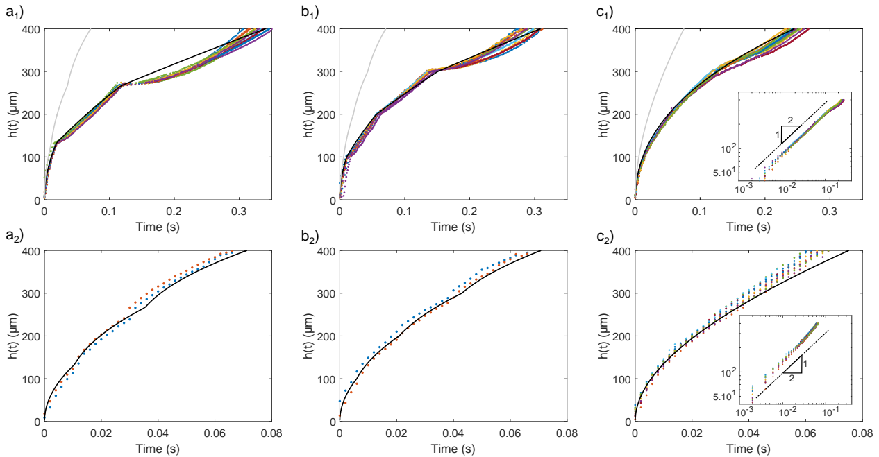
Figure 3.22: Kinetics of imbibition in channels with parabolic cross section varying from 8.1\mu\text{m} \times 400\text{nm} to 6\mu\text{m} \times 250\text{nm} : a) 3 steps channels, b) 4 steps channels, c) slope channels. Comparison between experiments, in dots, and theory in black line. Each color corresponds to a different experiment. Index 1 refers to imbibition from the shallowest to the deepest side and index 2 vice-versa. Note that for these figures, time seems to be more discrete only because the kinetics is faster (see the theoretical kinetics of imbibition in way 2 reported for comparison in figure of way 1 in light gray).
