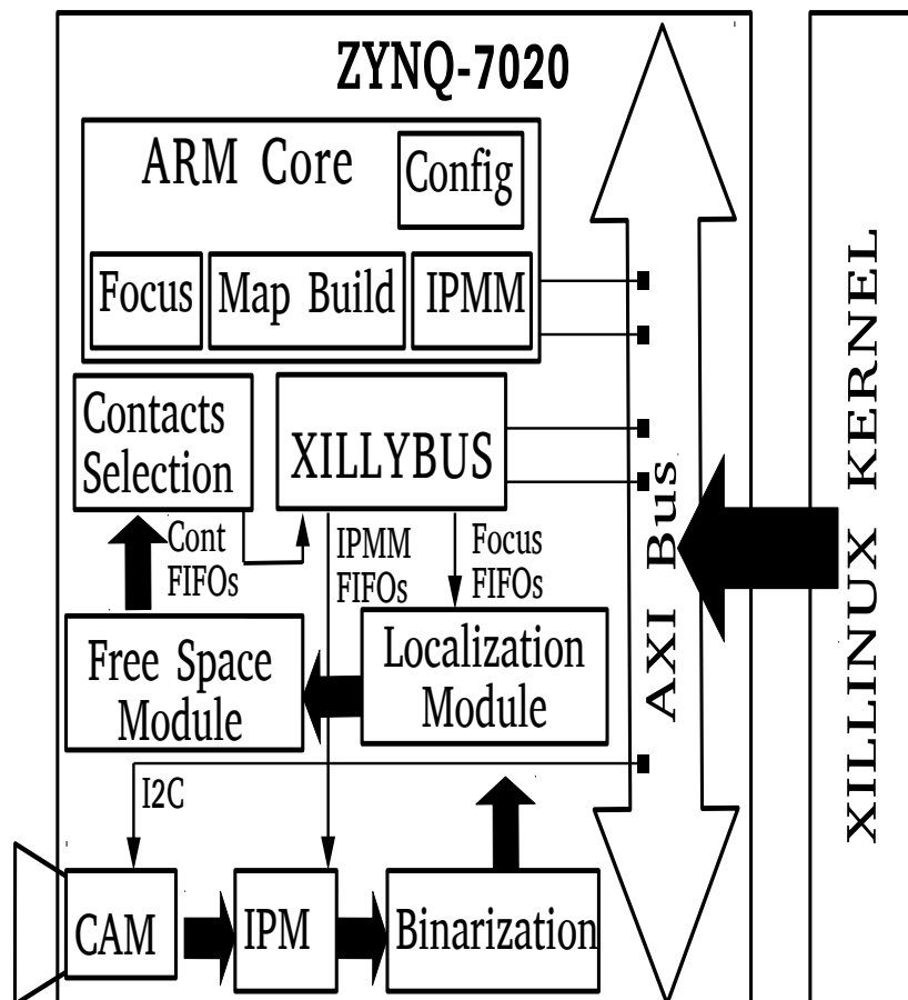
Figure 7.23: Occupancy system.
