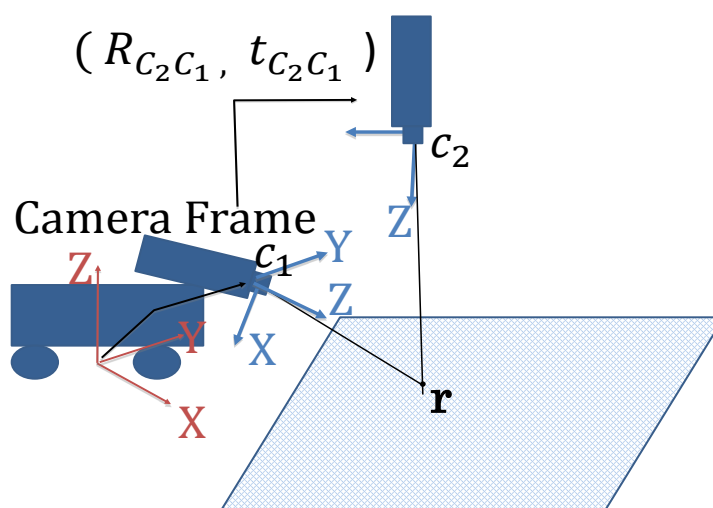
Figure 3.8: Bird's eye view transformation.
