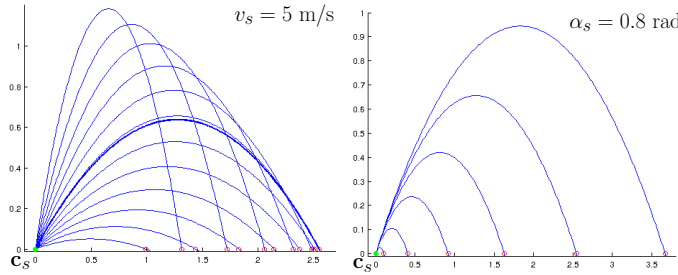
Figure 5.3: Accessible space from \mathbf{c}_s = (0 \ 0)^T when varying takeoff angle \alpha_s (left), or when varying initial velocity v_s (right). On left, the bold parabola leads to the maximal range at given initial velocity, and is obtained for \alpha_s = \frac{\pi}{4} .
