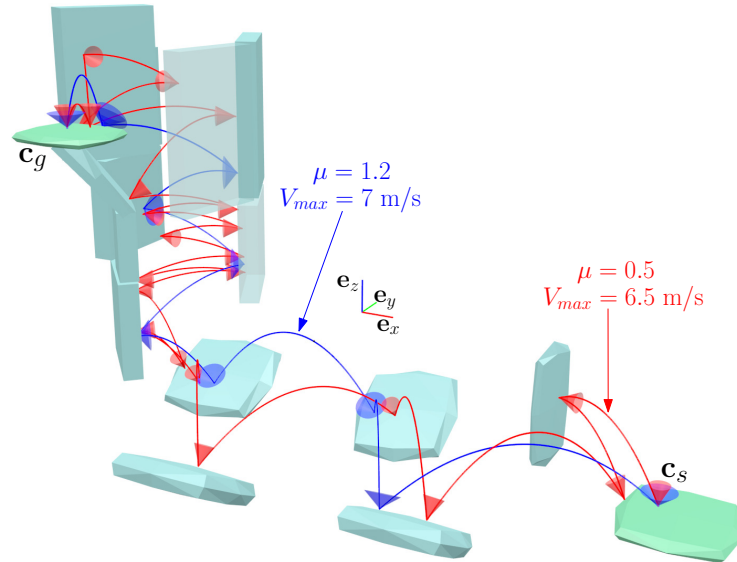
Figure 5.13: Full path planning results in an environment containing platforms and a chimney. The blue path is constrained by large cones, the red path by narrow cones. Reducing \mu prevents the creation of a parabola linking two low platforms with the same inclination. Number of triangles: 696.
