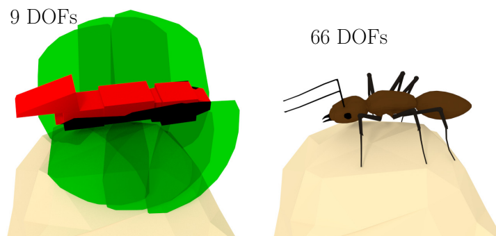
Figure 6.3: Illustration of a necessary condition for contact creation. If the trunk bounding box is collision-free (left–red), and the reachable workspaces of the limbs are in collision with the environment (left–green), we assume that a contact configuration can be created between the effectors and the environment (right).
