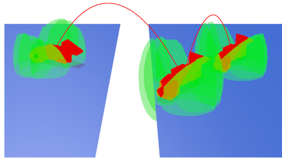
Figure 6.4: Sequence of parabola paths for an ant reduced model. The takeoff velocity limitation prevents the direct connection from start to goal, so a waypoint is found by the planner to solve the problem. At each waypoint configuration, the accessible workspaces of the legs are in collision with the environment. During the first jump, the robot is rotating to match the second parabola orientation.
