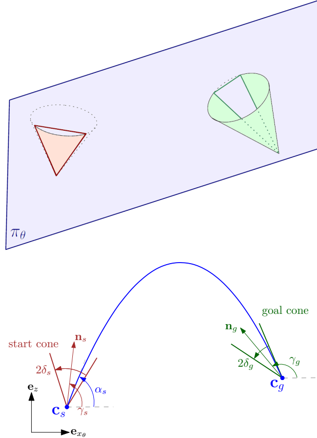
Figure 5.6: (Top) Representation of the intersection between \pi_\theta and two 3D cones. (Bottom) 2D cones resulting from the intersection and an example of parabola belonging to both cones.
