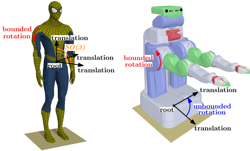
Figure 2.3: Examples of joints for a humanoid character and the PR2 robot.
