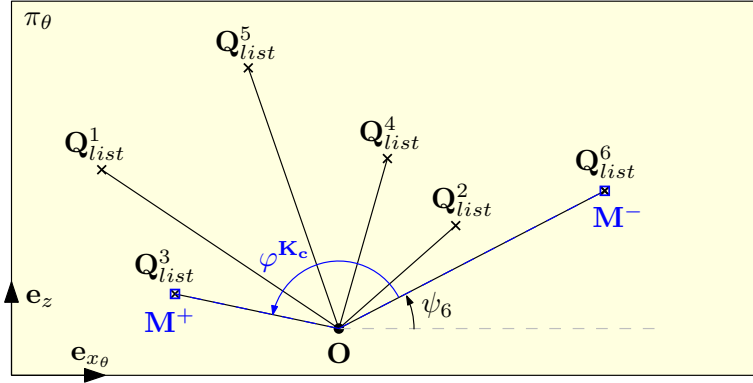
Figure A.4: Example of a convex cone \mathcal{K}_c delimited by (\mathbf{O}, \mathbf{OM}^+, \mathbf{OM}^-) and of half-apex angle \varphi^{\mathcal{K}_c} .
