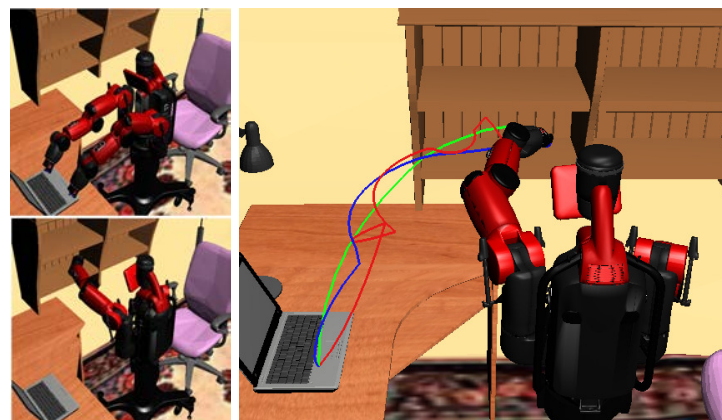
(c) Baxter-in-office
