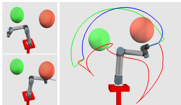
(c) UR5-with-spheres
