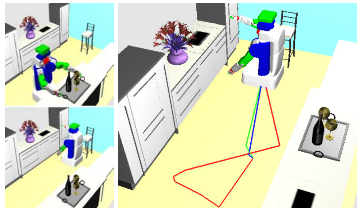
(b) PR2-in-kitchen-2
