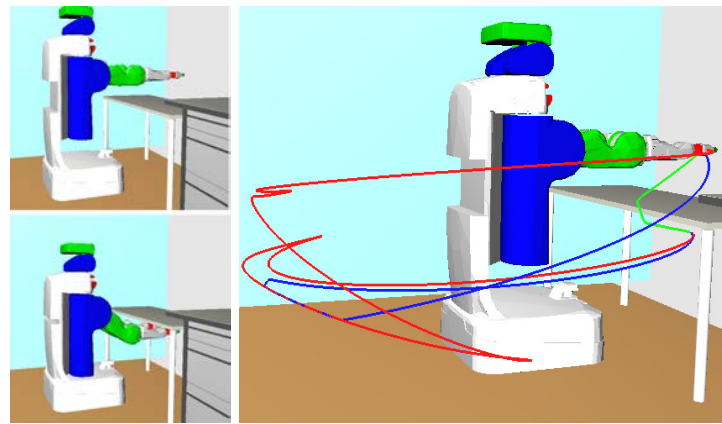
(a) PR2-in-kitchen-1
