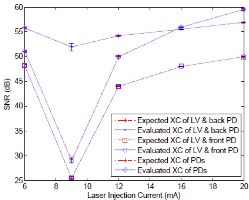
Fig. 4.13: SNRs of the cross-correlation of the OFI signal pairs as a function of laser injection current (solid blue: obtained values, and dashed red: expected values).
