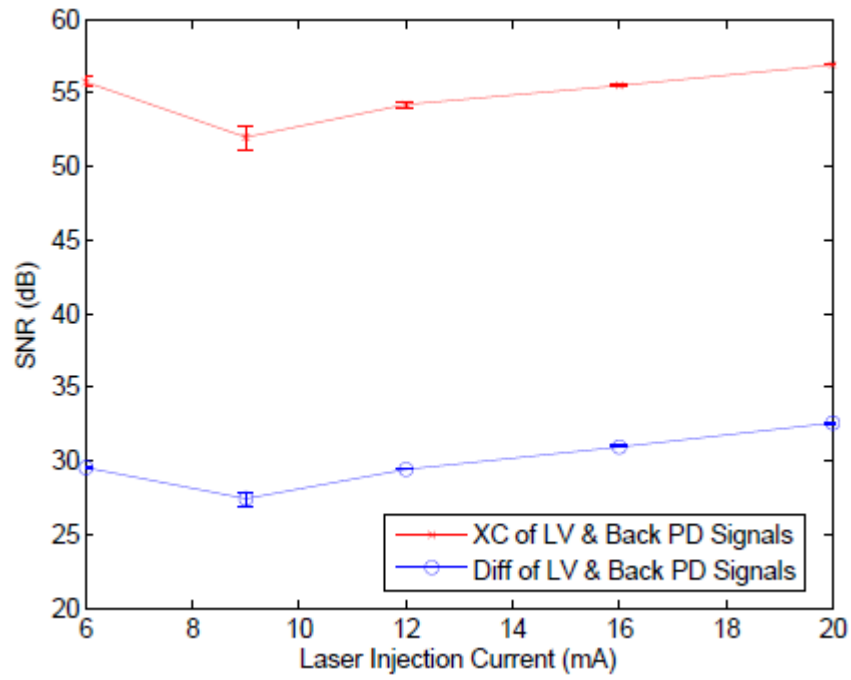
Fig. 4.17: Comparison of the SNRs of both the cross-correlation and the difference of the LV and back PD signals as a function of the laser injection current (solid red: cross-correlation and solid blue: difference).
