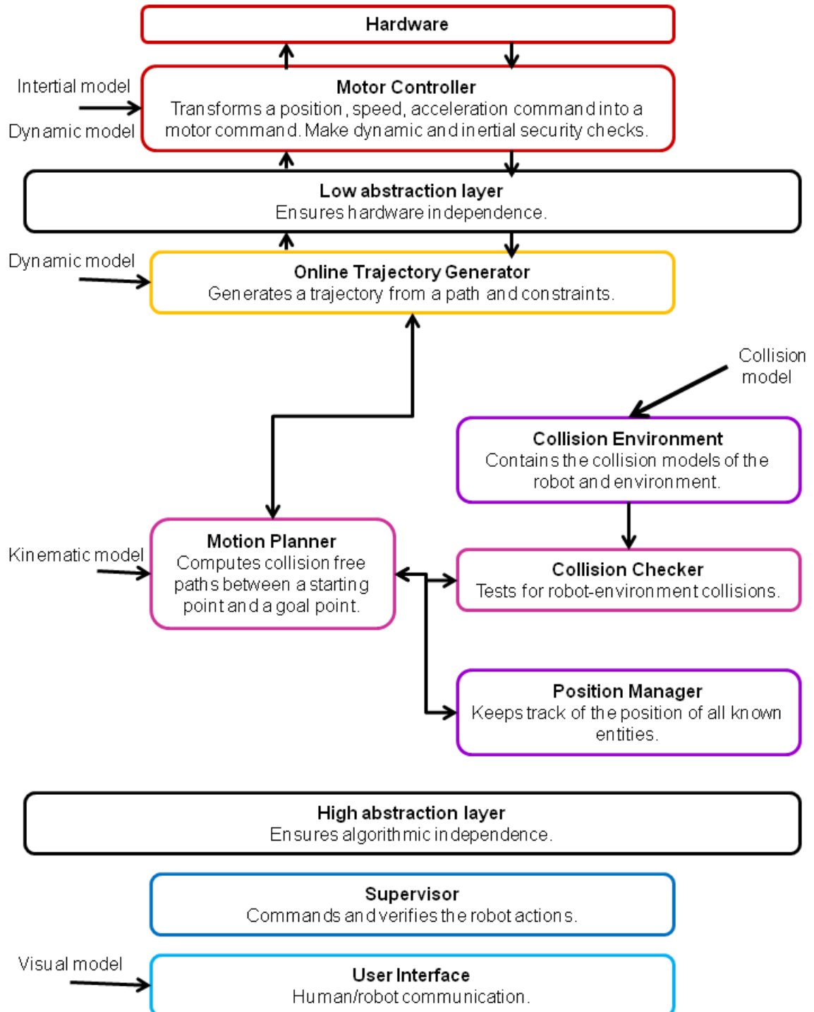
Figure 8.16: A robotic software architecture.
