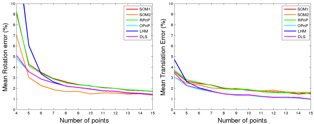
Figure 5.3: Mean rotation and translation errors for a noise with standard deviation of two pixels and a number of points going from 4 to 15.
