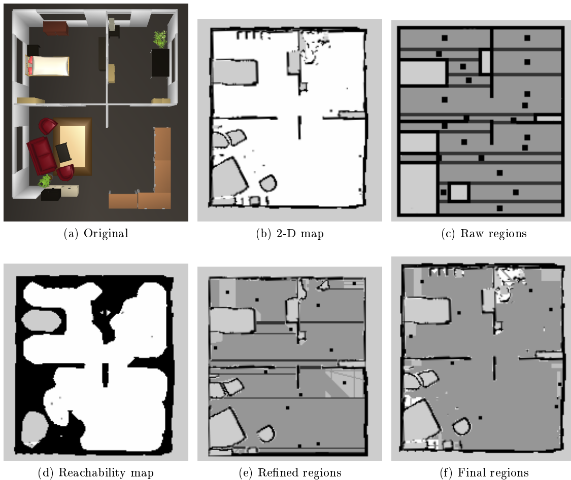
Figure 6.2: View point selection process. The boundaries of the 2-D map are extended, horizontally in this case. Small and unreachable regions are removed. Regions with similar view points are merged.
