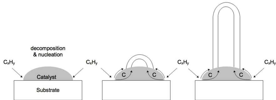
Figure 1.4: Base-growth model. C_xH_y represents hydrocarbon as carbon precursor. The scheme is inspired by the Ref.[25] and depicts the growth of DWCNTs.
