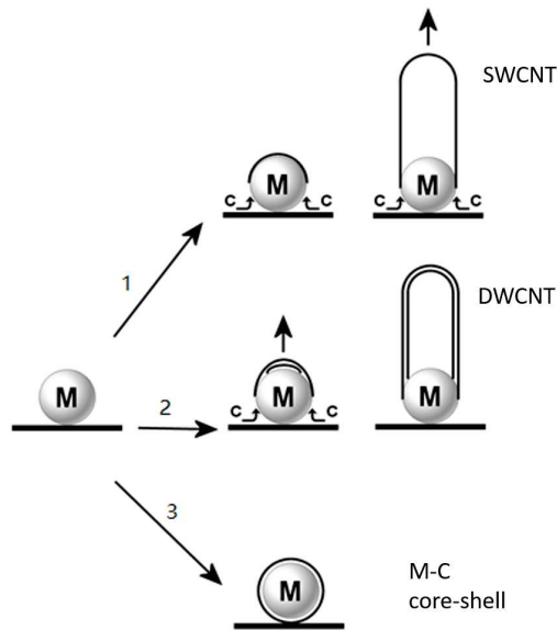
Figure 1.1: DWCNTs synthesis via CCVD method under metal nanoparticles (M). The process described in the text mainly produces DWCNTs according to the process depicted in route 2.
