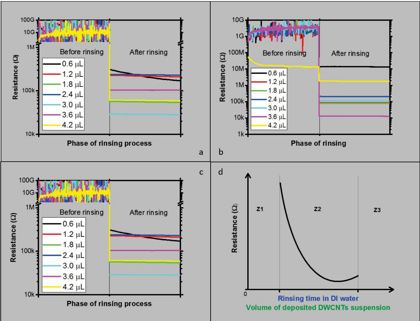
Figure 1.14: a), b), and c) are the resistance variation of 7 sensors of three different devices. d) shows a mode of resistance evolution with rinsing times and resistance differences between each electrode of one device after rinsing depending on the amount of deposited raw DWCNTs. Z1, Z2 and Z3 represent uncertainty zone, regular zone and undetermined zone, respectively, corresponding to the volume of deposited DWCNTs suspension axis label.
