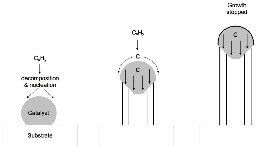
Figure 1.5: Tip-growth model. C_xH_y represents hydrocarbon as carbon precursor. The scheme is inspired by Ref.[26] and depicts the growth of DWCNTs.
