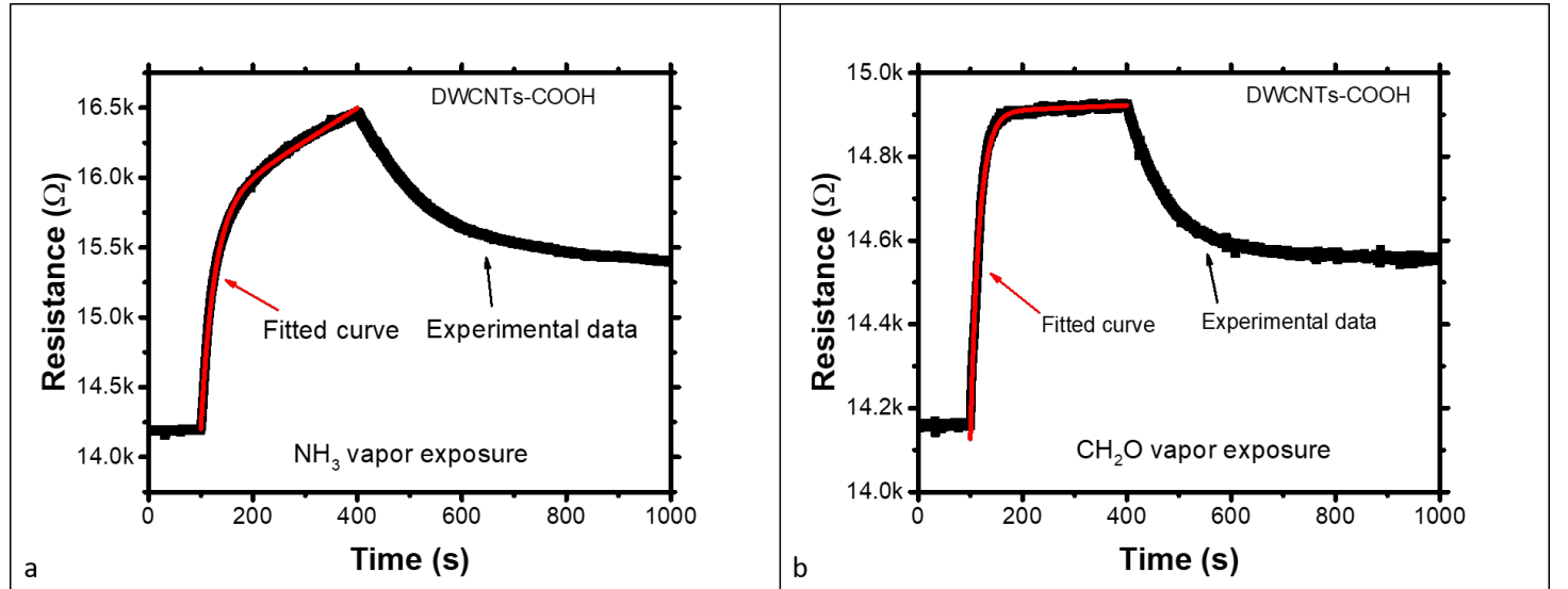
Figure 2.25: An oxidized DWCNTs sensor's resistance evolution (black curves) upon ammonia (a) and formaldehyde (b) vapor exposures with fitted curves (red) using model 2.9.
