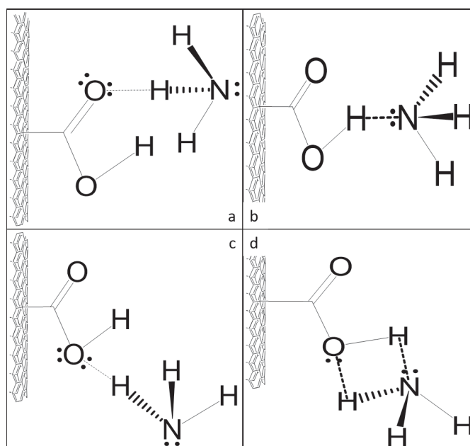
Figure 2.13: Other possible configuration hydrogen binding between carboxyl group and ammonia.
