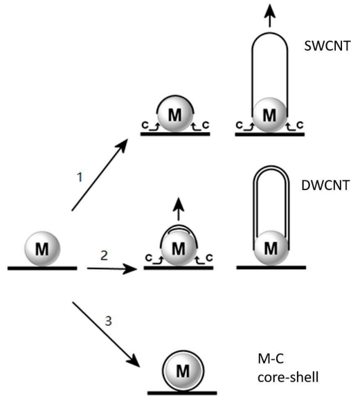
Figure 1.1: DWCNTs synthesis via CCVD method under metal nanoparticles (M). The process described in the text mainly produces DWCNTs according to the process depicted in rout 2.
