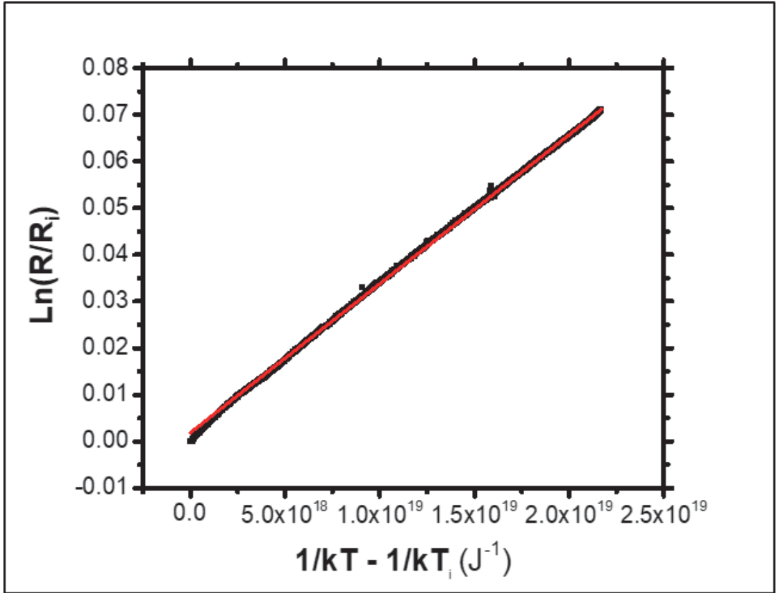
Figure 1.19: The electrical measurements of an oxidized DWCNTs sensor's resistance (black) which is plotted in the form of equation 1.4. The red curve is fitted with equation 1.4.
