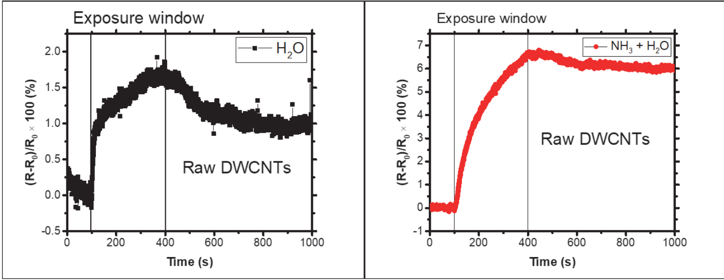
Figure 2.8: A raw DWCNTs sensor's response to water vapor (left) and ammonia solution vapor (right). R_0 is the initial resistance before exposure which is ca. 91\text{ k}\Omega while R is the real-time resistance.
