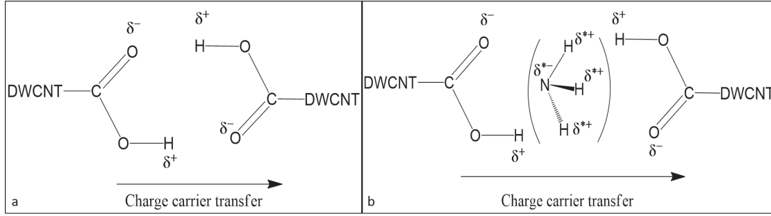
Figure 2.14: The junction of polar interaction before (a) and after (b) adsorbing an ammonia molecule. Assuming the charge carrier flow from left to right DWCNTs when electric field applied.
