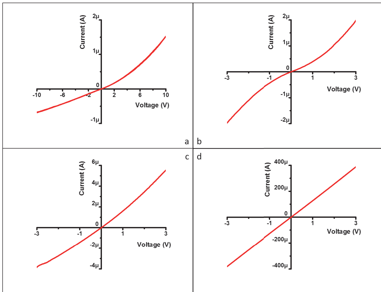
Figure 1.15: I-V characterization of raw DWCNTs based sensors. (a) and (b) sensors exhibit Schottky diode behaviour, while (c) and (d) show ohmic behaviour.
