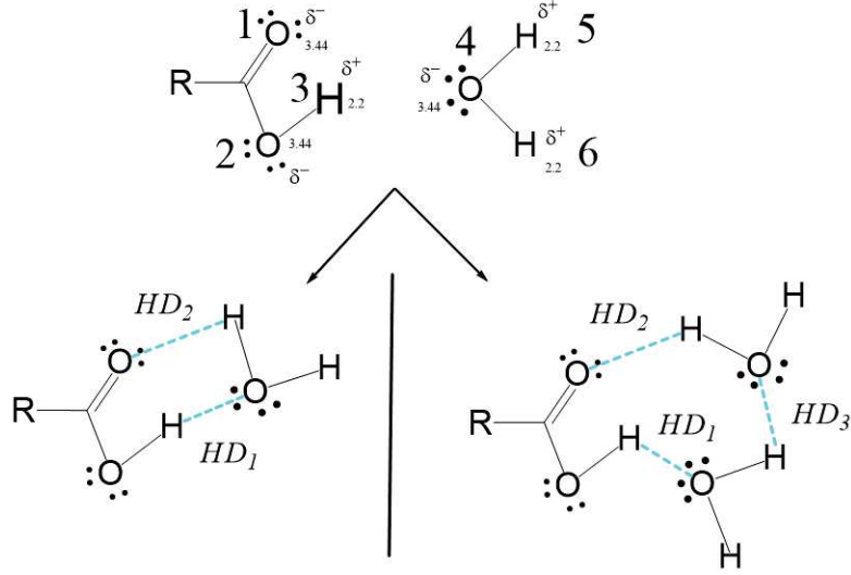
Figure 2.15: (a) The partial charge configuration of carboxyl group on DWCNT and water molecule. The integers are the index of atoms and the decimal are the electronegativity of corresponding element. \delta with superscripts '+' and '-' denote the positive and negative partial charge. (b) and (c) are the hydrogen binding configurations of two of the most stable isomers as calculated in Ref. [15]
