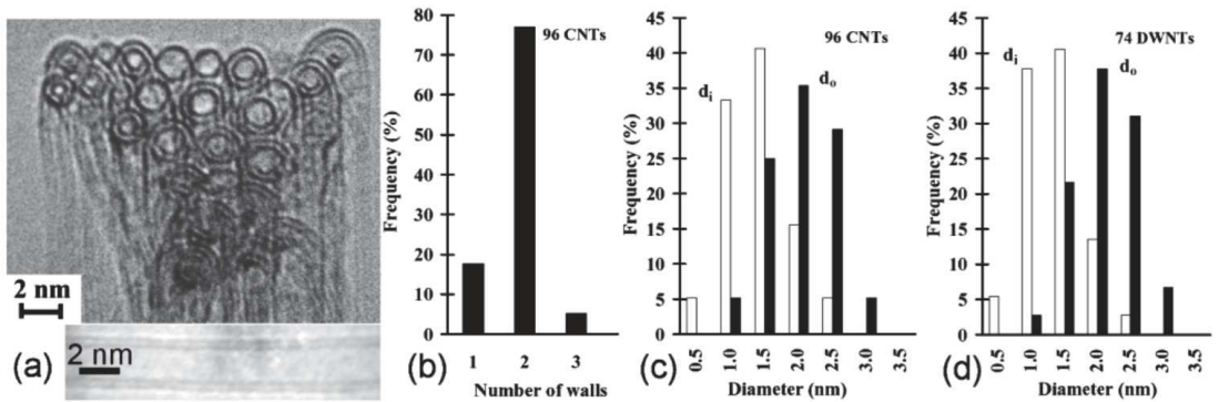
Figure 1.2: (a) HRTEM image of DWCNTs and (b) distribution of the numbers of walls for the whole population (established from 96 individual CNTs). Distribution of inner ( d_i ) and outer ( d_o ) diameter for the whole population of (c) CNTs and for (d) DWCNTs only.
