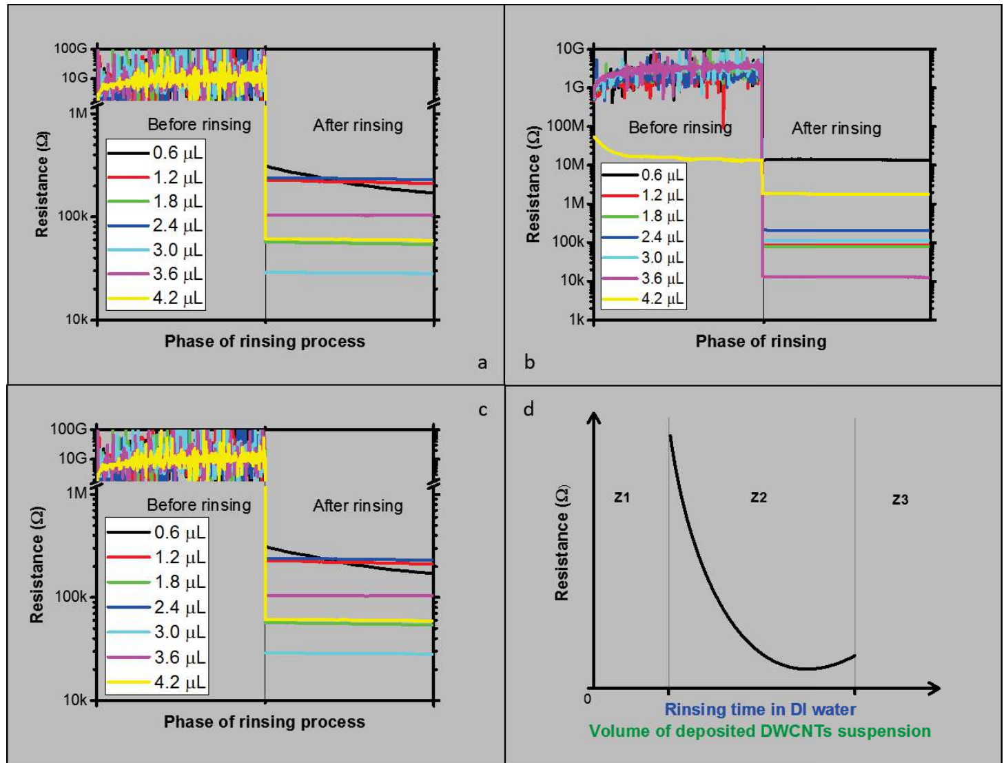
Figure 1.14: a), b), and c) are the resistance variation of 7 sensors of three different devices. d) shows a mode of resistance evolution with rinsing times and resistance differences between each electrode of one device after rinsing depending on the amount of deposited raw DWCNTs. Z1, Z2 and Z3 represent uncertainty zone, regular zone and undetermined zone, respectively, corresponding to the volume of deposited DWCNTs suspension axis label.
