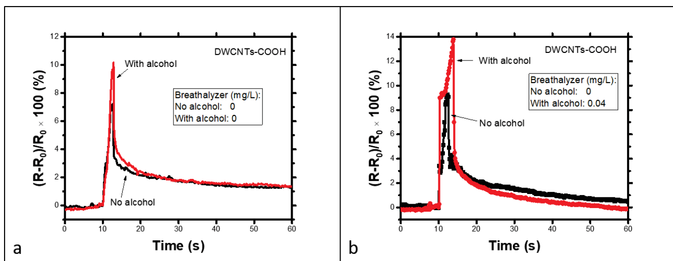
Figure 1.2: The signal of an oxidized DWCNTs sensor to the second alcohol drinking test. The insert box show the corresponding readings by the commercial breathalyzer.
