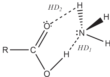
Figure 2.12: Most stable configuration isomer formed by carboxylic acids and ammonia. Two hydrogen bonds are formed, ' HD_1 ' and ' HD_2 '.
