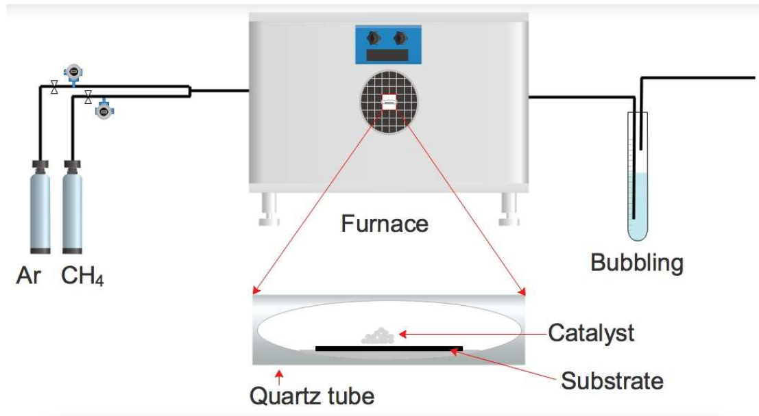
Figure 1.3: Illustration of a typical catalyst vapor deposition process of SWCNTs fabrication as described in the work of A. M. Cassell et. al[19].
