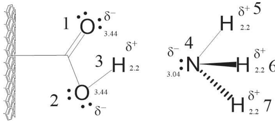
Figure 2.11: Polarization in carboxyl group and ammonia molecule. The integer is the index of atoms. Notes that the 5, 6 and 7 hydrogen atoms are equivalent to each other here. The decimal numbers next to atoms are corresponding element electronegativities. As oxygen and nitrogen have stronger electronegativity, they have negative potential in each dipole. \delta with superscripts '+' and '-' denote the positive and negative partial charge.
