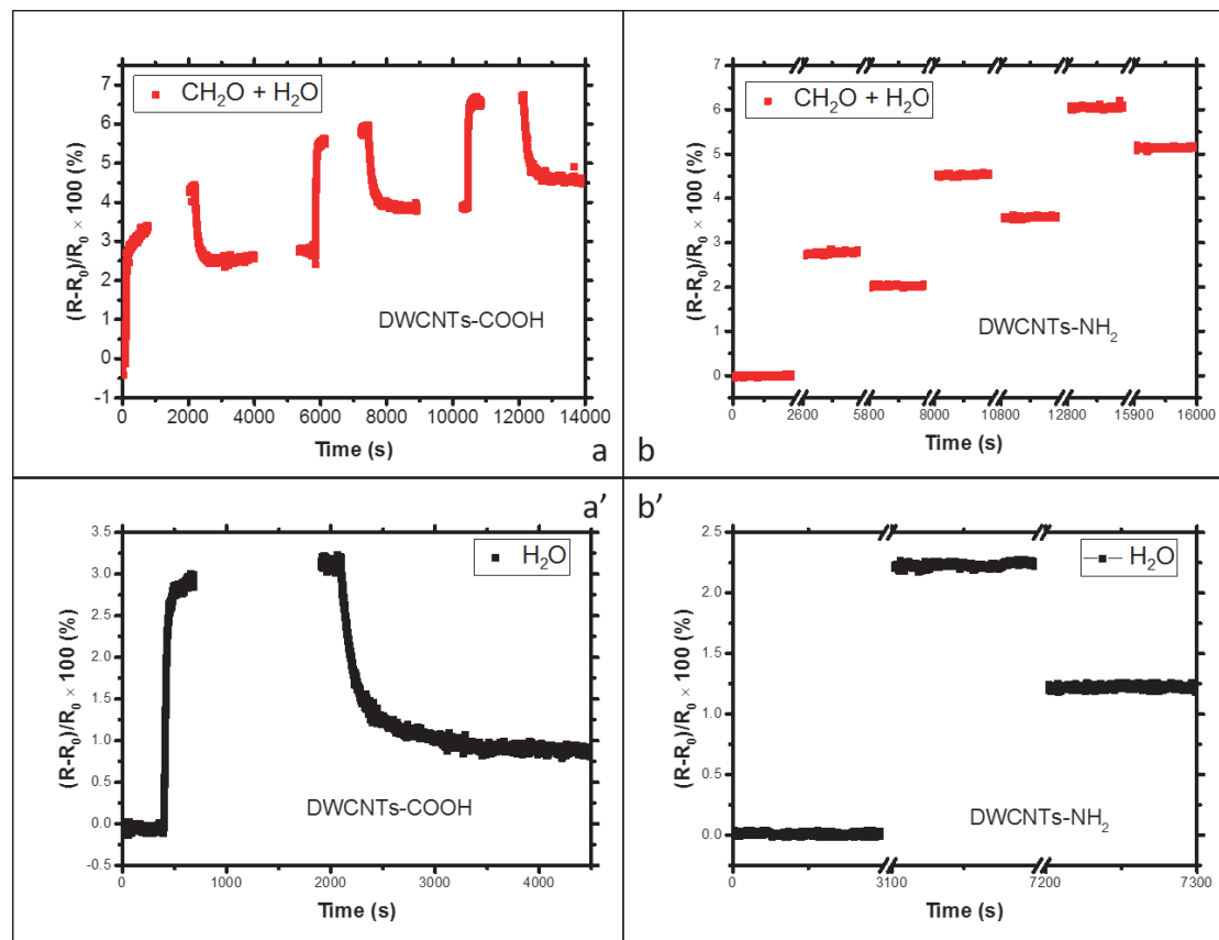
Figure 2.22: The signal of oxidized DWCNTs sensor (a) and aminated DWCNTs sensor (b) to repeated exposures of formaldehyde vapor. (a') and (b') are response of corresponding sensor to DI water vapor exposure, respectively. The R and R_0 are the resistance of sensor in real-time and initial resistance, respectively.
