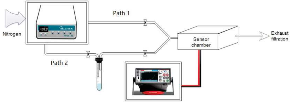
Figure 2.1: Schematic of gas exposure and detection setup.
