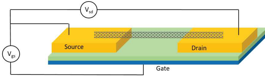
Figure 2.1: Scheme of NTFET based gas sensor.
