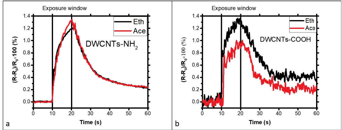
Figure 2.3: The signal of aminated (a) and oxidized (b) DWCNTs gas sensors to ethanol and acetone vapor exposure. The terms 'Eth' and 'Ace' in legend represent response to ethanol vapor and acetone vapor, respectively. R_0 is the initial resistance before exposure which is ca. 4 kΩ while R is the real-time resistance.
