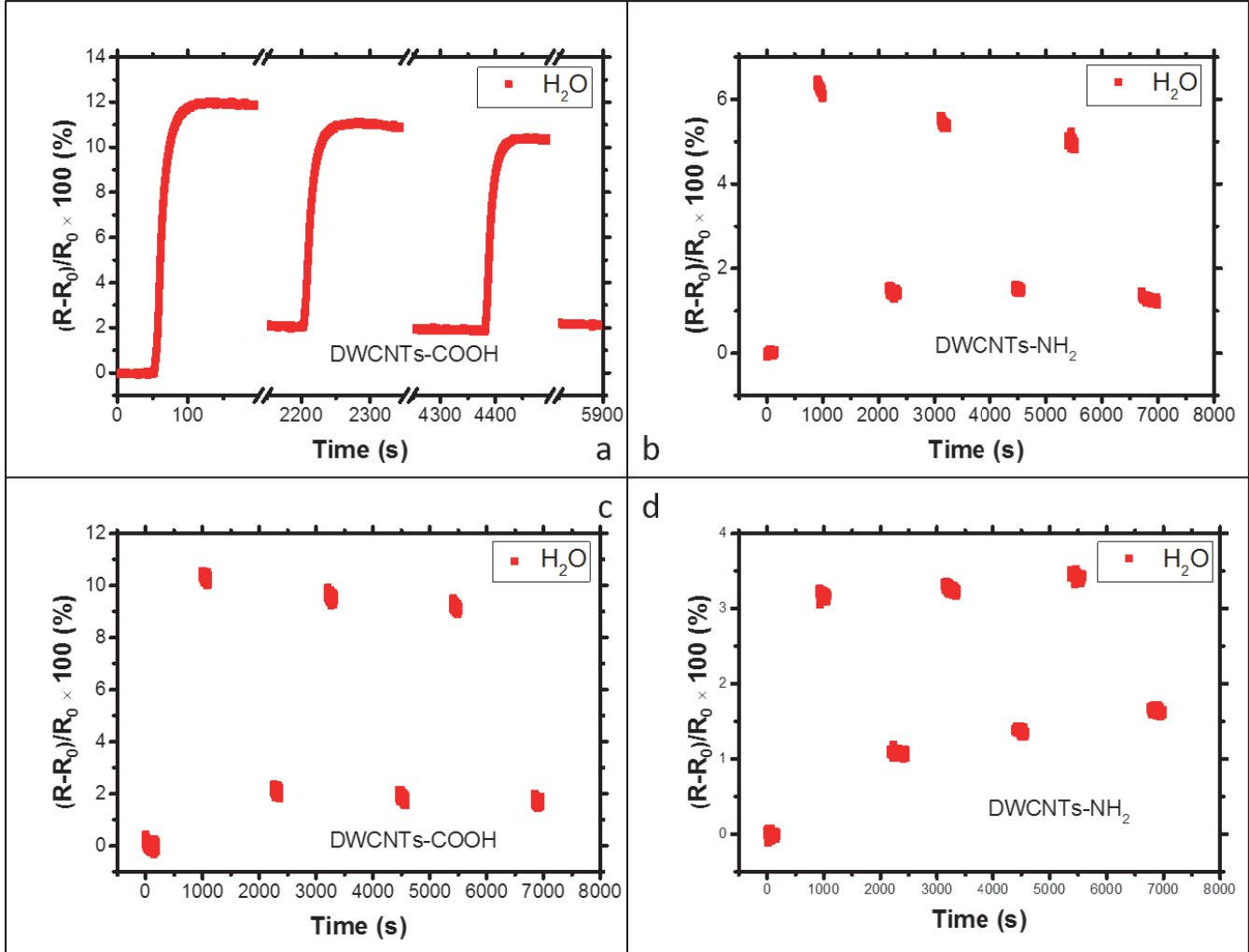
Figure 2.18: Control experiment of repeated exposure to 5690 ppm water vapor (in the absence of ammonia vapor) on oxidized DWCNTs gas sensors ((a), (c)) and aminated DWCNTs gas sensors ((b), (d)) corresponding to the sensors in Figure 2.17.
