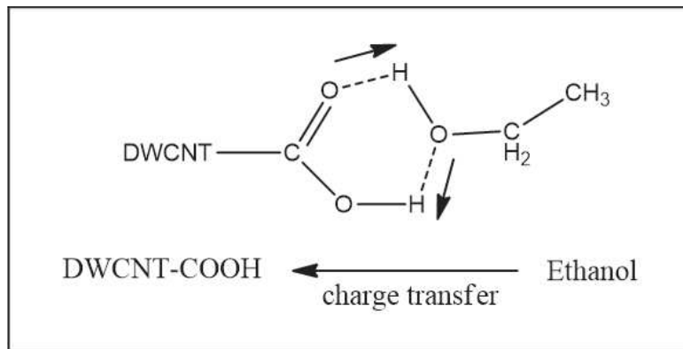
Figure 2.7: Hypotheses of hydrogen bond between ethanol and carboxyl group of oxidized DWCNTs. The arrows indicate negative charge transfer through hydrogen bond.
