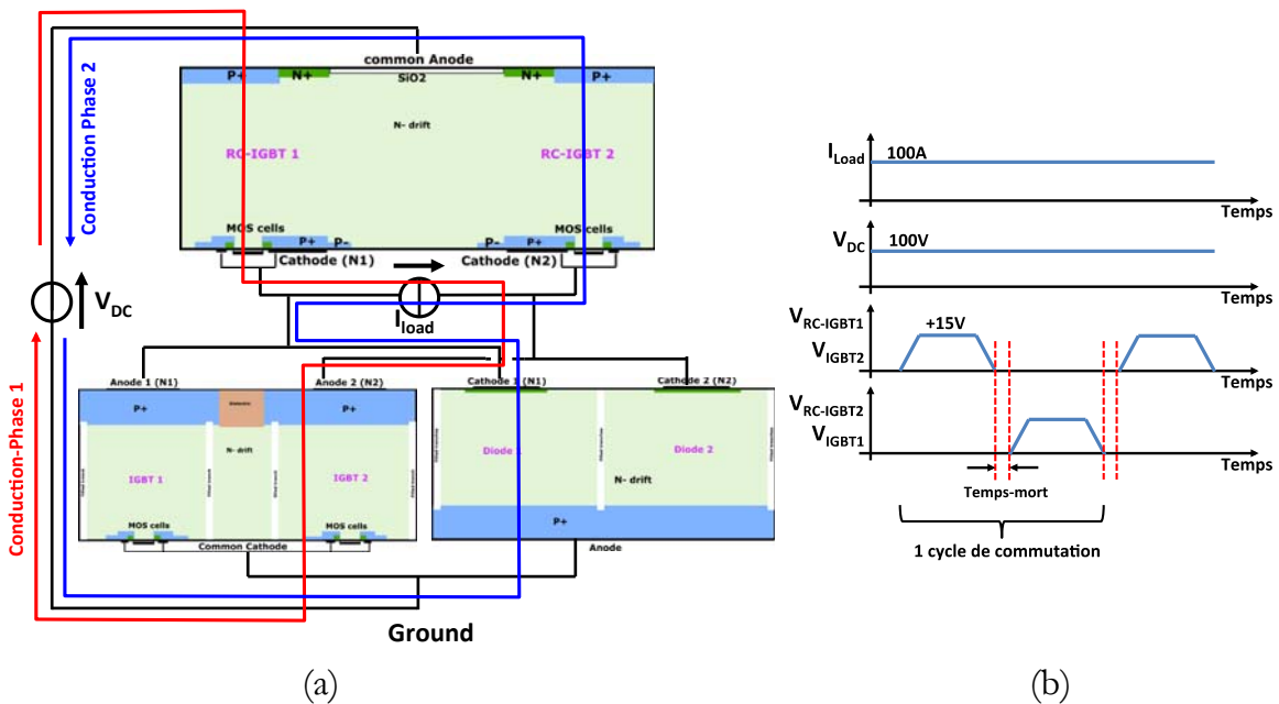
Figure 84 : (a) pont en H – mode tri-puce, (b) chronogrammes de commande (tension grille-cathode = +15 V, temps-mort = 1 µs, I_{load} = 100 A)
