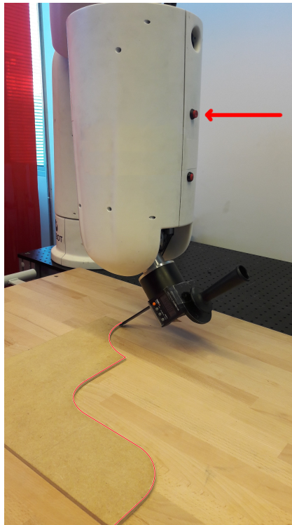
Figure 5.15: Programming task setup. The path to follow is highlighted in red
