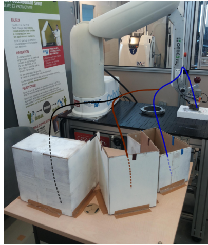
Figure 6.1: Multiple Virtual Guides created in the robot workspace for the Pick-and-Place Experiment presented in [Raiola 2017a]. The task consisted in taking 6 discs from the robot's workstation and insert them inside specific boxes identified with 3 different colors: blue, brown and black. For each box there were two discs with a piece of tape of the same color.
