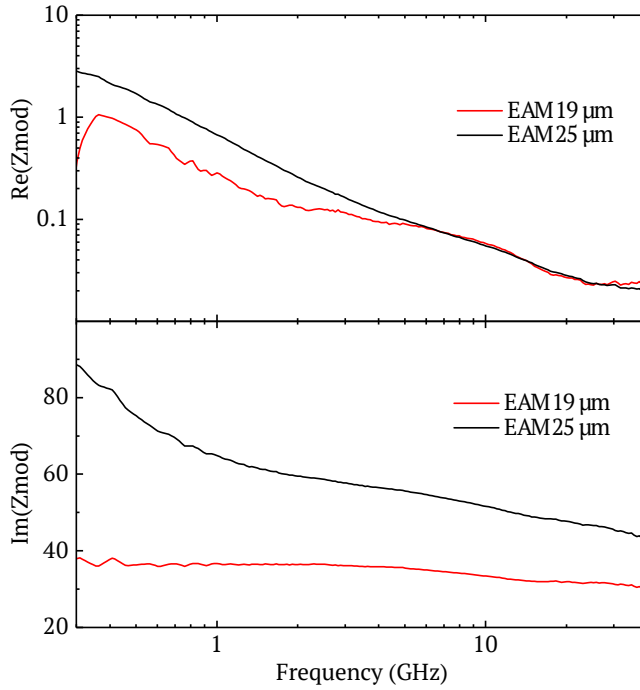
Figure 5.19: Resistance and capacitance of 19 \mu\text{m} (red) and 25 \mu\text{m} (black) EAM.
