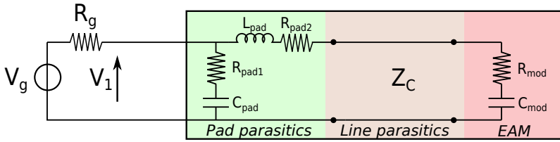
Figure 5.17: Microstrip line access for EAM-VCSEL device.
