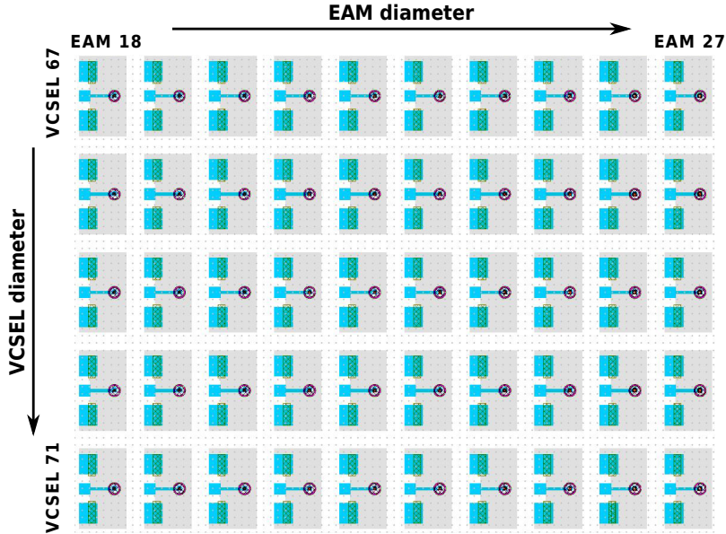
Figure 4.22: Unitary block of devices. EAM diameters are between 18\ \mu\text{m} and 27\ \mu\text{m} and VCSEL mesa diameters between 67\ \mu\text{m} and 71\ \mu\text{m} . This block is then repeated with different line length and pad areas.
