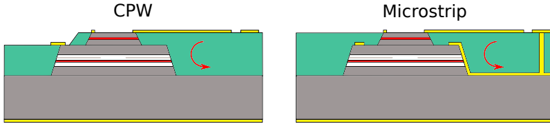
Figure 4.18: Schematic crossview of the EAM-VCSEL with CPW access (left) or Microstrip line (right). The coupling is represented by the red arrow
