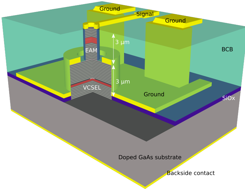
Figure 4.20: Global view of the EAM-VCSEL device
