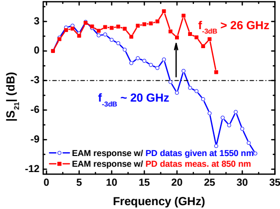
Figure 5.12: High frequency characterization of the 27 μm-EAM, cut access of 50μm, with the photodiode response given by the supplier at 1550 nm (in blue) and with the extraction of our measurements at 850 nm (red)
