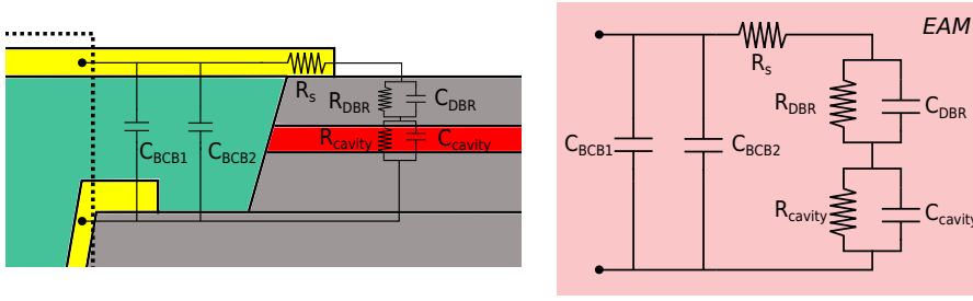
Figure 5.20: Equivalent circuit of the EAM from the end of the line de-embedding to cavity.
