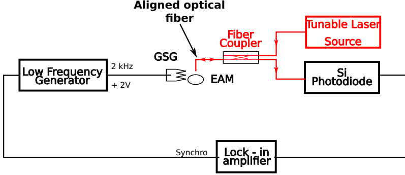
Figure 5.1: Schematic of the set up used for the optical alignment of a single mode fiber on top of the EAM for an optimum light injection. In red the optical paths, in black the electrical paths.
