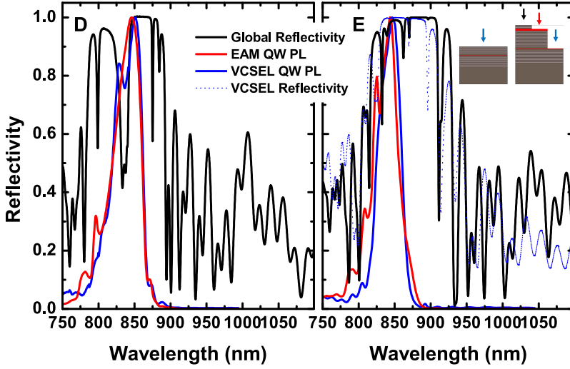
Figure 3.11: Rellectivity and Photoluminescence of the QWs of the EAM-VCSEL structures. Global reflectivity (black), PL of the EAM QW (red), PL of the VCSEL QW (blue) and for the wafer E, VCSEL reflectivity (dashed blue).
