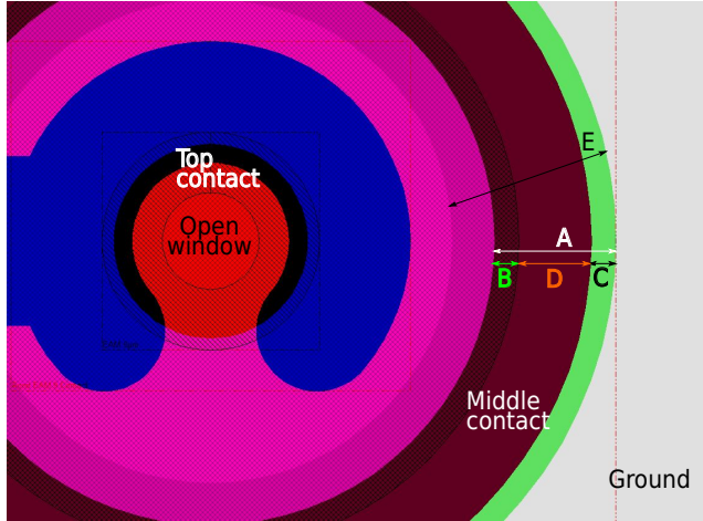
Figure 8.1: Global top view of the different masks
