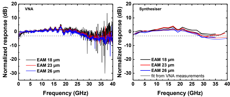
Figure 5.15: Comparaison of electro-optic characterization with a VNA (left) and with a synthesiser (right). For a better comparison, fits of the VNA measurements are also plotted with the synthesiser results.
