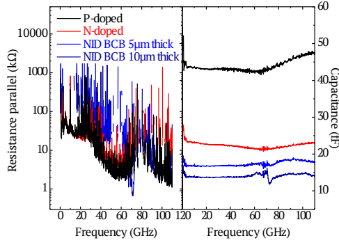
Figure 4.16: Resistance parallel and capacitance extracted from the CPW access measurements
