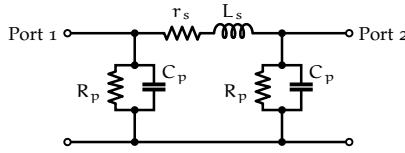
Figure 4.14: \Pi equivalent lumped network used to model Thru structures.
