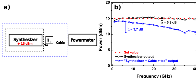
Figure 5.4: Power calibration of the RF synthetiser set to +15 dBm alone (black curve) and with the system "bias tee + cable" (blue curve).
