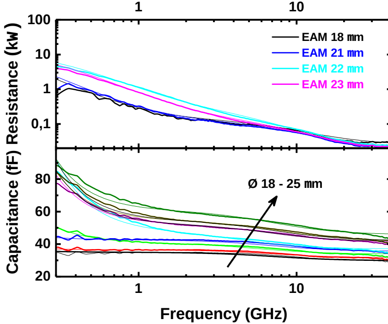
Figure 5.21: Real and Imaginary part of the EAM impedance fitted with our double R//C model.
