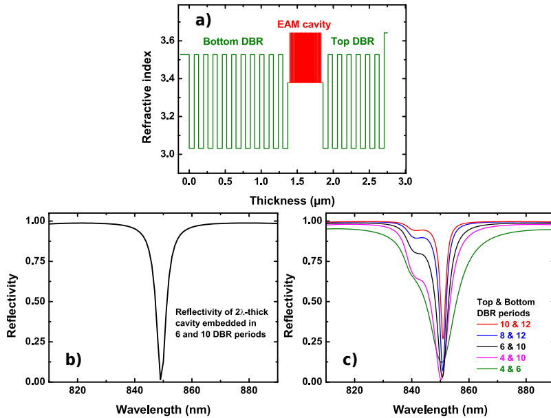
Figure 2.9: MQW embedded in an Asymmetric Fabry-Perot structure. a) Refractive index variation along the structure, b) reflectivity of an ASFP of 6 and 10 DBR periods without consideration of the absorption phenomena c) Reflectivity with the absorption for different couples of parameters
