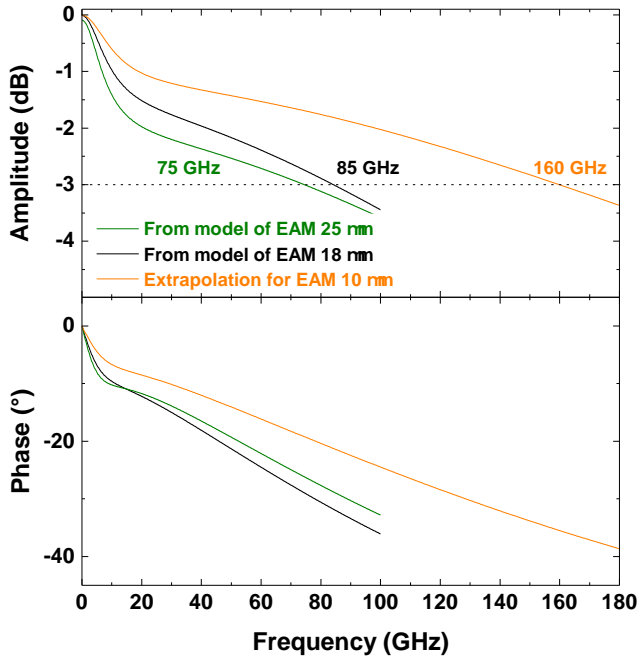
Figure 5.25: Transfert functions calculated from our electrical model for 18 \mu\text{m} (black) and 25 \mu\text{m} (green). In orange is represented the extrapolation for a 10 \mu\text{m} -EAM.
