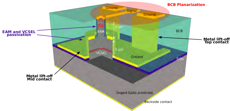
Figure 3.13: Global view of the EAM-VCSEL device. Technological difficulties are highlighted around the schematic.
