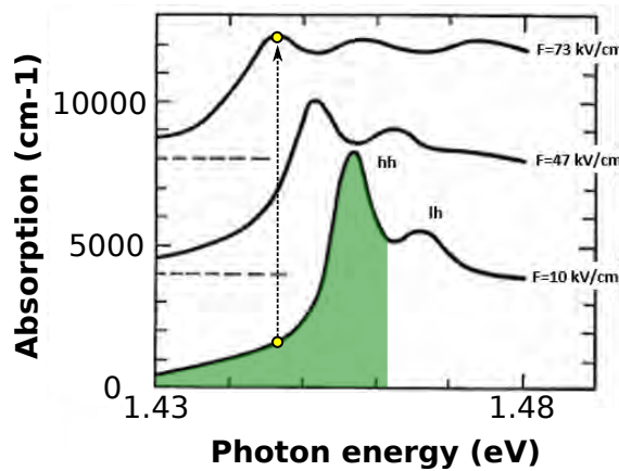
Figure 2.5: Schematic of the Quantum Confined Stark Effect (QCSE) in a MQW structure of 50 QWs under electric field. Light and heavy hole exciton peak position are denoted. The green area corresponds to the higher modulation depth that can be achieved; so it highlights our area of interest. From [59]
