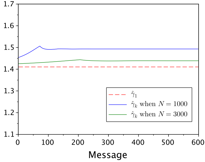
Figure 4.5: The value of \hat{\gamma}_1 and \hat{\gamma}_k with N = 1000; 3000 , \mu = 0.8 , \lambda = 0.4 . We see that when N is large, the duration of time that a relay keeps a message is the same for all messages.
