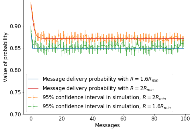
Figure 5.4: Analytical probability of message delivery and simulated probability for different values of \bar{R} .
