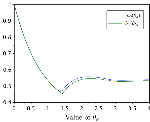
Figure 4.6: The function m_0 and function h_1 with N = 3000 , \mu = 0.8 , \lambda = 0.4 .
