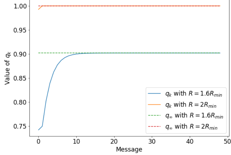
Figure 5.3: Value of q_k and its limiting value.
