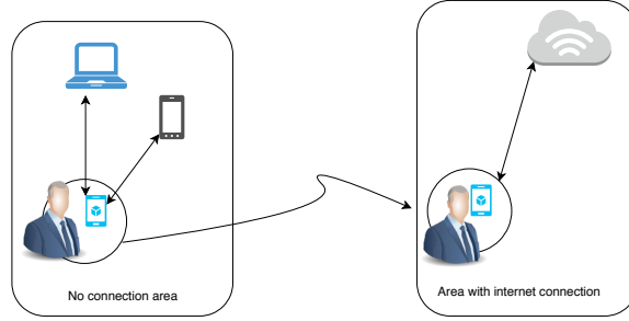
Figure 1.7: In areas where there is no network connectivity, nodes forward data to relays who may move to connected areas. Once a relay has an Internet connection, it sends data to a server.
