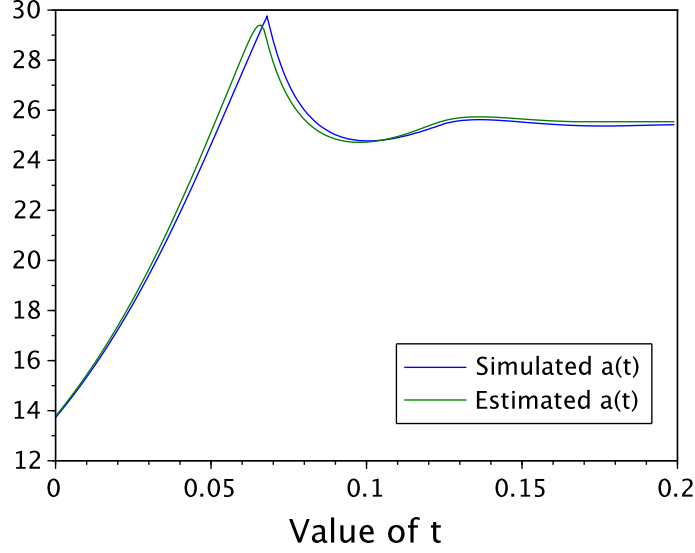
Figure 4.7: The estimated \hat{a}(t) and the analytical a(t) with N = 3000 , \mu = 0.4 , \lambda = 0.8 .
