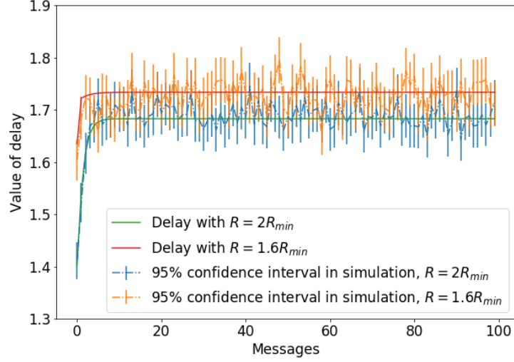
Figure 5.5: Analytical delay and simulated delay.
