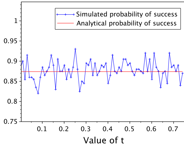
Figure 4.3: The simulated probability and its analytical value with N = 800 , \mu = 0.5 , \lambda = 0.3 .
