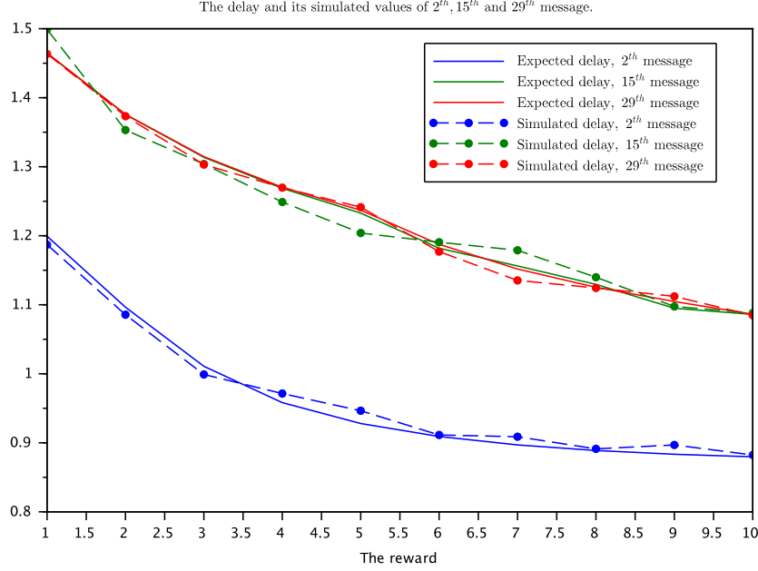
Figure 3.9: Comparison of the theoretical expected delays of 2 nd , 15 th and 29 th messages against expected delays obtained through simulations.
