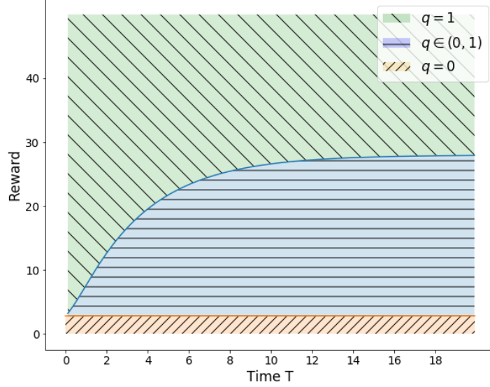
Figure 5.1: Equilibrium acceptance probability q_1 as a function of R and T , when the values of the parameters are as follows: \mu = 0.5 , \lambda = 0.3 , C_r = C_d = 2 and C_s = 0.4 .
