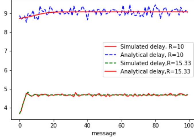
Figure 3.7: Theoretical expected delays of first 30 messages compared against values obtained through simulations for R = 10 and R = 15.33 .
