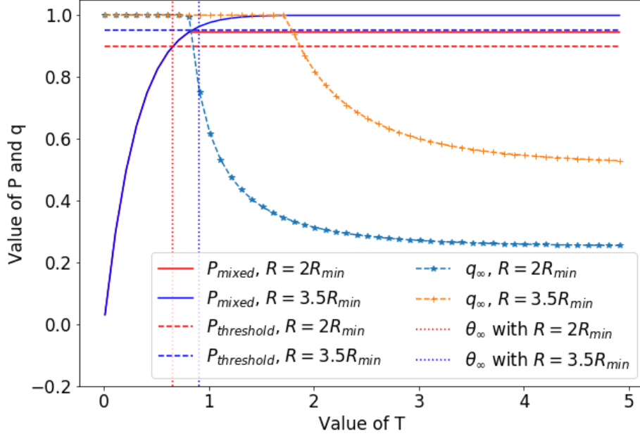
Figure 5.7: The message delivery probability in mixed strategy and threshold strategy, with \mu = 0.4 , C_d = C_r = 2 , C_s = 0.4 , N = 10 and \lambda = 1.5 .
