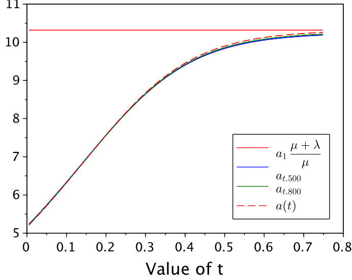
Figure 4.2: The behavior of \hat{a}(t) when \mu = \lambda = 0.4 and N = 500; 800 .
