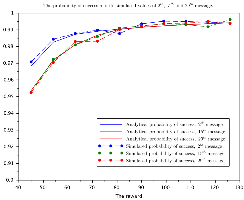
Figure 3.8: Comparison of the theoretical probabilities of success of 2^{nd} and 29^{th} messages against expected probabilities of success obtained through simulations.
