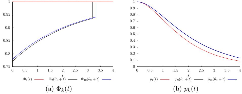
Figure 3.5: Evolution of \Phi_k(t) and p_k(t) with k .
