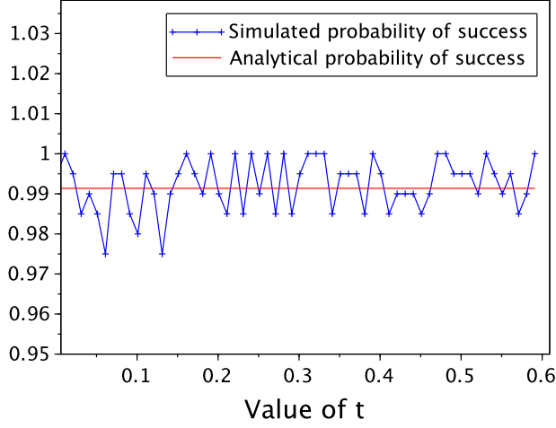
Figure 4.8: The simulated probability of success and its analytical value with N = 1000 , \mu = 0.8 , \lambda = 0.4 .
