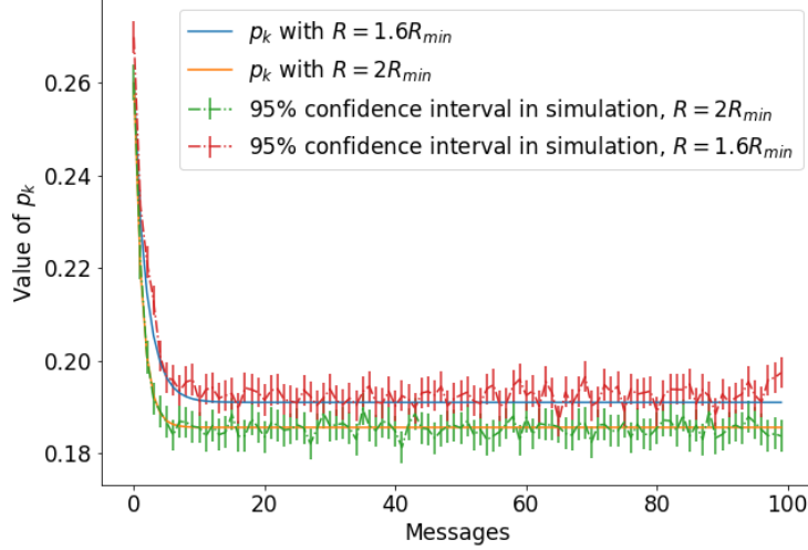
Figure 5.2: Value of p_k in two cases with R = 1.6R_{min} and R = 2R_{min} as well as their 95% confidence interval.
