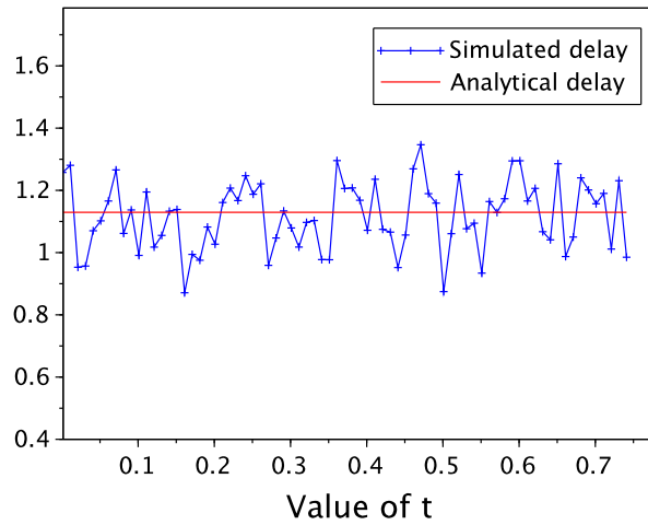
Figure 4.4: The simulated delay and its analytical value with N = 800 , \mu = 0.5 , \lambda = 0.3 .
