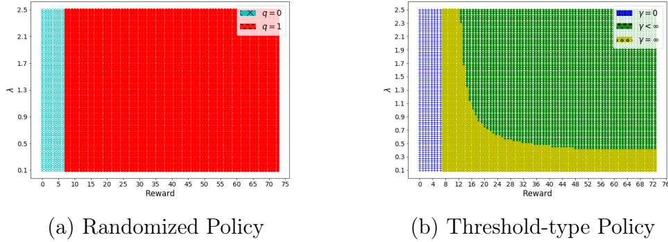
Figure 5.6: Randomized and threshold-type policies as functions of R and \lambda for the first message when T = \theta_1 . The values of the parameters are \mu = 0.4 , C_d = 2 , C_r = 4 , C_s = 0.5 and N = 3 .
