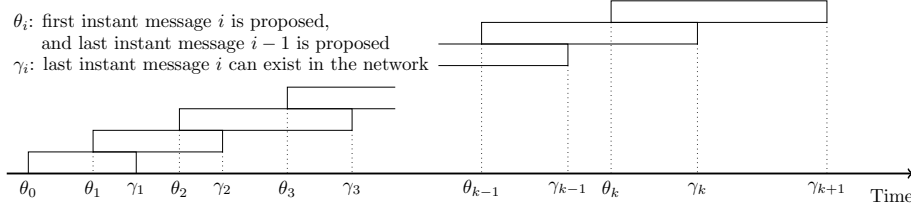
Figure 3.1: Message injection policy of the source at the symmetric Nash equilibrium.
