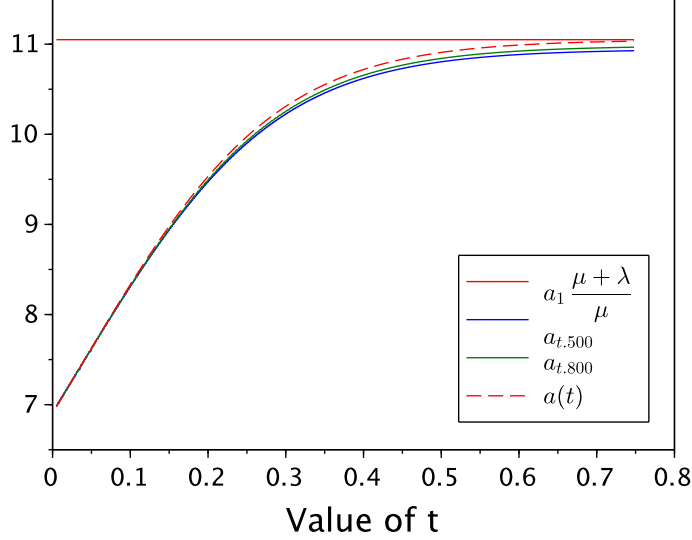
Figure 4.1: The behavior of \hat{a}(t) when \mu = 0.5 , \lambda = 0.3 and N = 500; 800 .
