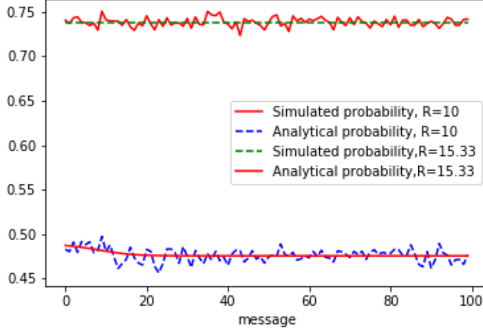
Figure 3.6: Theoretical values of the probability of success and its values obtained through simulations for R = 10 ( \gamma = \infty ) and for R = 15.33 ( \gamma < \infty ).
