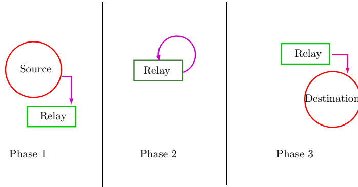
Figure 1.6: In two-hop network, we do not allow a node to forward the message to other nodes. It will store the message until it meets the destination and transmits the message.
