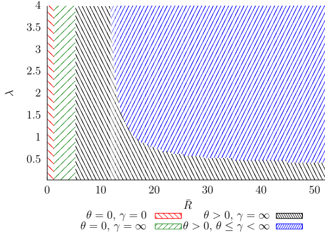
Figure 3.4: Existence of a symmetric Nash equilibrium for 3 relays.
