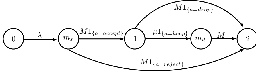
Figure 3.3: Controlled Markov Chain for relay i .
