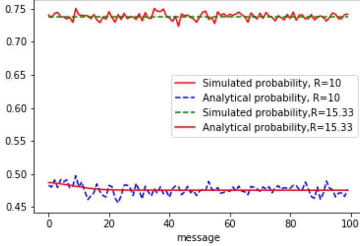
Figure 3.6: Theoretical values of the probability of success and its values obtained through simulations for R = 10 ( \gamma = \infty ) and for R = 15.33 ( \gamma < \infty ).
