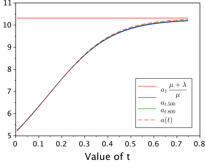
Figure 4.2: The behavior of \hat{a}(t) when \mu = \lambda = 0.4 and N = 500; 800 .
