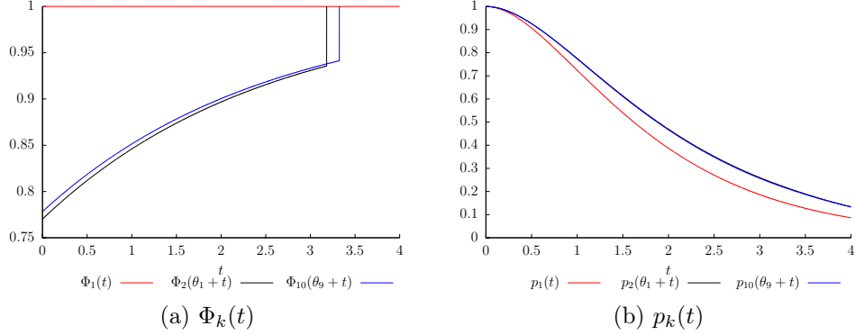
Figure 3.5: Evolution of \Phi_k(t) and p_k(t) with k .
