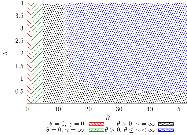
Figure 3.4: Existence of a symmetric Nash equilibrium for 3 relays.
