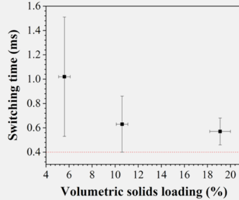
Fig. 8. Switching time as a function of the volumetric solids loading. The red dashed line corresponds to the ignition time of the nanothermites ignitor.
