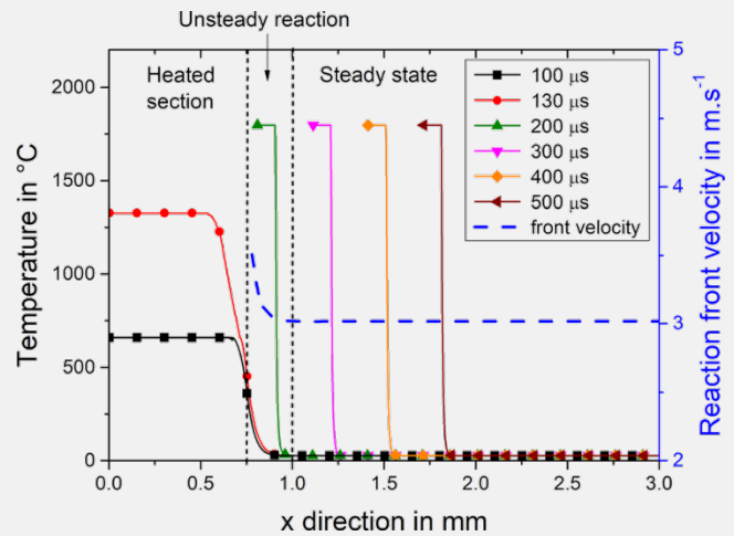
FIG. 5. Temperature profiles at selected times and the instantaneous reaction front velocity. The multilayer is composed of ten 300 nm 1:1 Al/CuO bilayers deposited on a polymer substrate, with \lambda_s = 0.1 \text{ W}\cdot\text{m}^{-1}\cdot\text{C}^{-1} .
