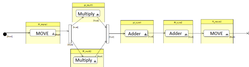
Fig. 6.19 Activity Diagram for the digital PI controller
