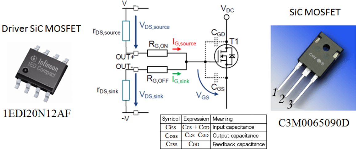
Fig. B.8 Selection driver SiC-MOSFET
