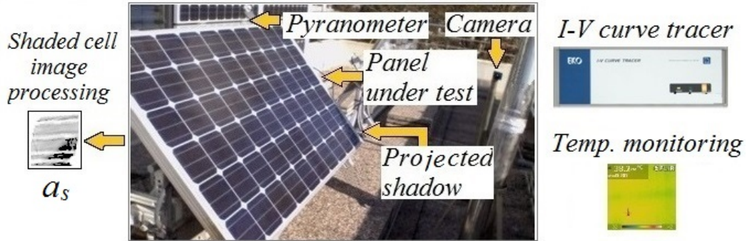
Fig. 3.14 Experimental setup
