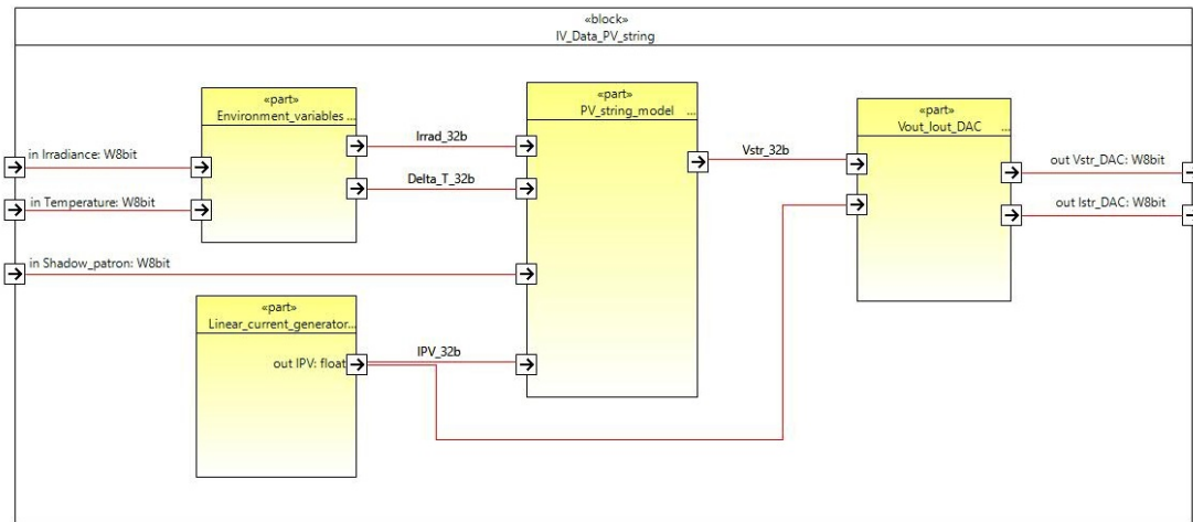
Fig. 5.7 Partial Internal Block Diagram for PV model emulation
