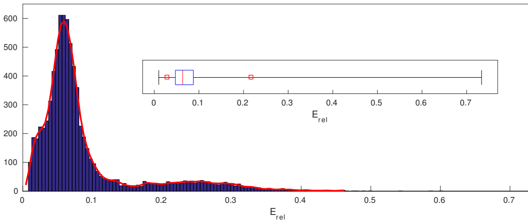
Figure 3.3: For the BVP in one dimension: the histogram of the distribution of the relative error for the 7,740 sub-optimal cases alongside with its box plot. In the later, the ends of the whiskers are the extremal values, the red squares are the 10th and 90th percentiles, the edges of the blue box are the first and third quartiles and the red segment inside the box is the median.
