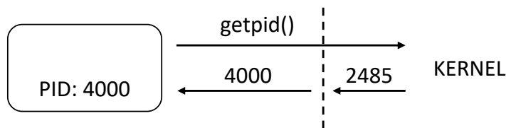
Figure 1.3 – Example of DMTCP plugin with getpid system call
