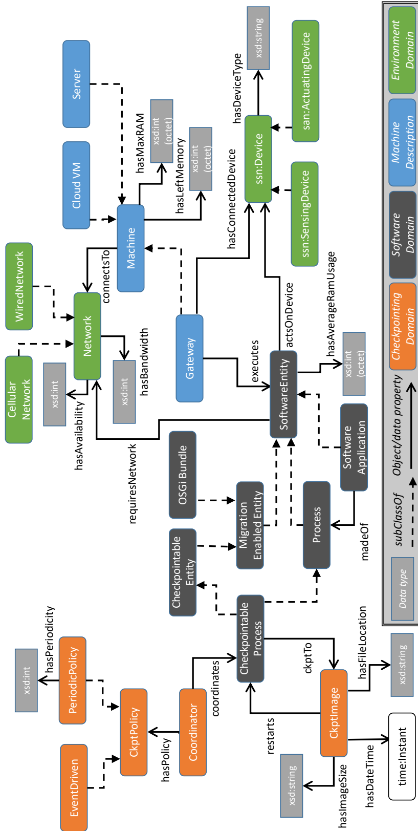
Figure 3.2 – Overview of the proposed ontology CplIoT-O
