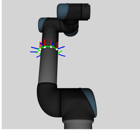
Figure 2.9: Skin cell sensors used in our experiments. They form a “ring” on the upper arm of the UR5 robot.
