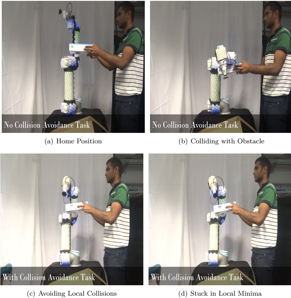
Figure 2.10: Test 1: Trajectory execution from home to pick location with and without collision avoidance task in the controller stack. (a) Initial state of the robot, i.e. Home position. (b) Trajectory execution without any collision avoidance task, leading to a collision with the obstacle. (c) Avoiding collision with the obstacle (d) The robot arm is stuck in local minimum.
