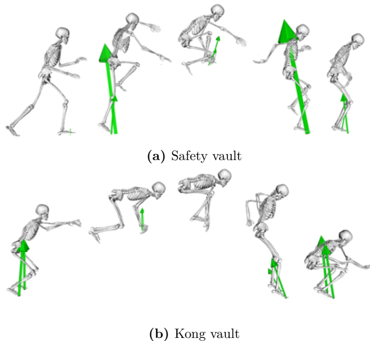
Figure 2.24: Vaulting techniques
