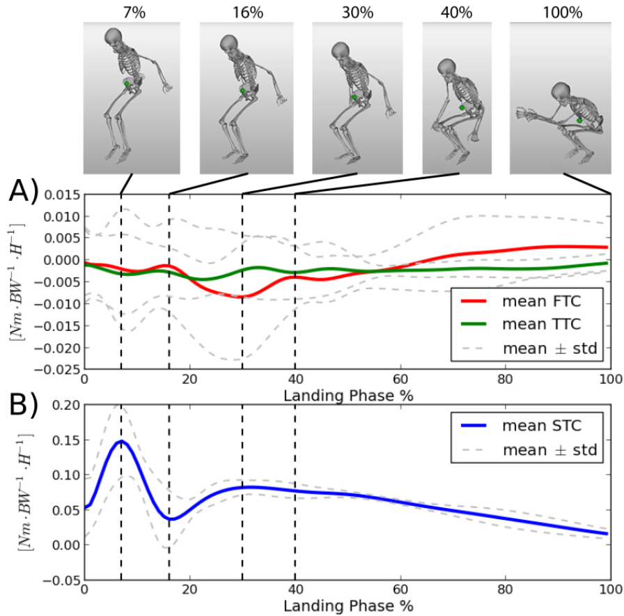
Figure 2.23: Mean ( \pm std) of the DAM around A-P (A, red), vertical (A, green) and M-L (B, blue) axes. In the top, snapshots of representative configurations extracted from the inverse kinematics computation, of a participant executing the precision landing technique.
