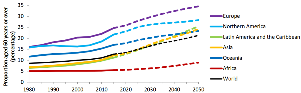
Figure 1.5: Percentage of the population aged 60 years or over, estimated for 1980-2017 and projected to 2050. Data source: World Population Prospects: the 2017 Revision .
