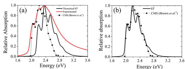
Figure 8. Experimental (rr-P3HT-Thin film) and vibrationally resolved simulated (8T) UV–vis absorption spectra at 83 K (a). \alpha Charge modulation spectroscopy (CMS) data extracted from ref 10 with g3data 1.5.4. Superimposition of the CMS spectrum and the 8T spectrum scaled by a factor of 0.94 (b).
