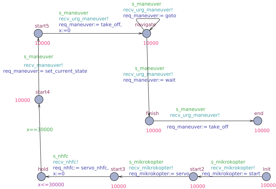
Figure 7.4: UPPAAL-SMC client (quadcopter).
