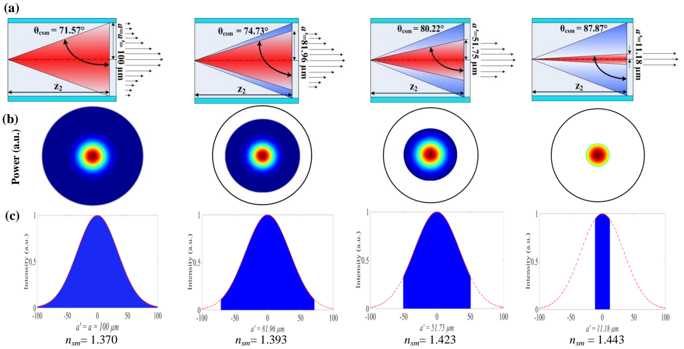
Figure 2.4. Evolution of optical power and intensity in the MMF RI sensor for various values of n_{sm} by modification of the critical angle, \theta_{csm} , for n_{cl} < n_{sm} < n_{co} : a) increasing n_{sm} will increase \theta_{csm} which reduces the acceptance angle of the propagating beam, b) power in transversal plane decreases for increasing n_{sm} , and c) illustrates decreasing optical intensity over different a' values obtained by Equation (2.17).
