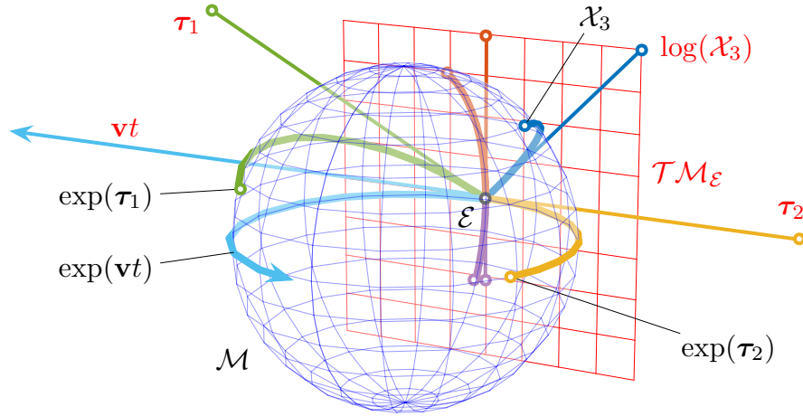
Figure 4.1: Representation of the relation between the Lie group and the Lie algebra. The Lie algebra \mathcal{T}\mathcal{M}_\mathcal{E} (red plane) is the tangent space to the Lie group’s manifold \mathcal{M} (here represented as a blue sphere) at the identity \mathcal{E} . Through the exponential map, each straight path \mathbf{v}t through the origin on the Lie algebra produces a path \exp(\mathbf{v}t) over the manifold which runs along the respective geodesic. Conversely, each element of the group has an equivalent in the Lie algebra. This relation is so profound that (nearly) all operations in the group, which is curved and nonlinear, have an exact equivalent in the Lie algebra, which is a linear vector space. Though the sphere in \mathbb{R}^3 is not a Lie group (we just use it as a representation that can be drawn on paper), that in \mathbb{R}^4 is, and describes the group of unit quaternions —see Fig. 4.3.
