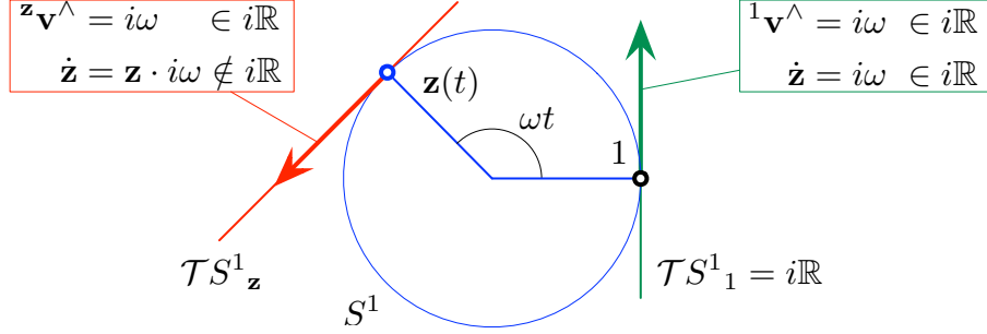
Figure 4.4: Let a point \mathbf{z} \in S^1 move at constant rotation rate \omega , \mathbf{z}(t) = \cos \omega t + i \sin \omega t . Its velocities when passing through 1 and \mathbf{z} are in the respective tangent spaces, \mathcal{T}S^1_1 and \mathcal{T}S^1_z . In the case of \mathcal{T}S^1_z , the velocity is \dot{\mathbf{z}} = \mathbf{z} i \omega = -\omega \sin \omega t + i \omega \cos \omega t when expressed in the global coordinates, and {}^z\mathbf{v}^\wedge = i\omega when expressed locally. Their relation is given by {}^z\mathbf{v}^\wedge = \mathbf{z}^{-1}\dot{\mathbf{z}} = \mathbf{z}^*\dot{\mathbf{z}} . In the case of \mathcal{T}S^1_1 , this relation is the identity {}^1\mathbf{v}^\wedge = \dot{\mathbf{z}} = i\omega . Clearly, the structure of all tangent spaces is i\mathbb{R} , which is the Lie algebra. This is also the structure of \dot{\mathbf{z}} at the identity, and this is why the Lie algebra is defined as the tangent space at the identity.
