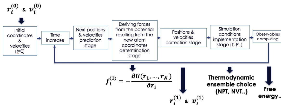
FIGURE 2.5: Molecular dynamics algorithm
