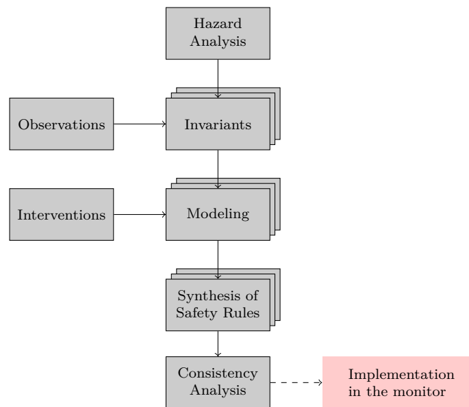
Figure 1.4: SMOF process
