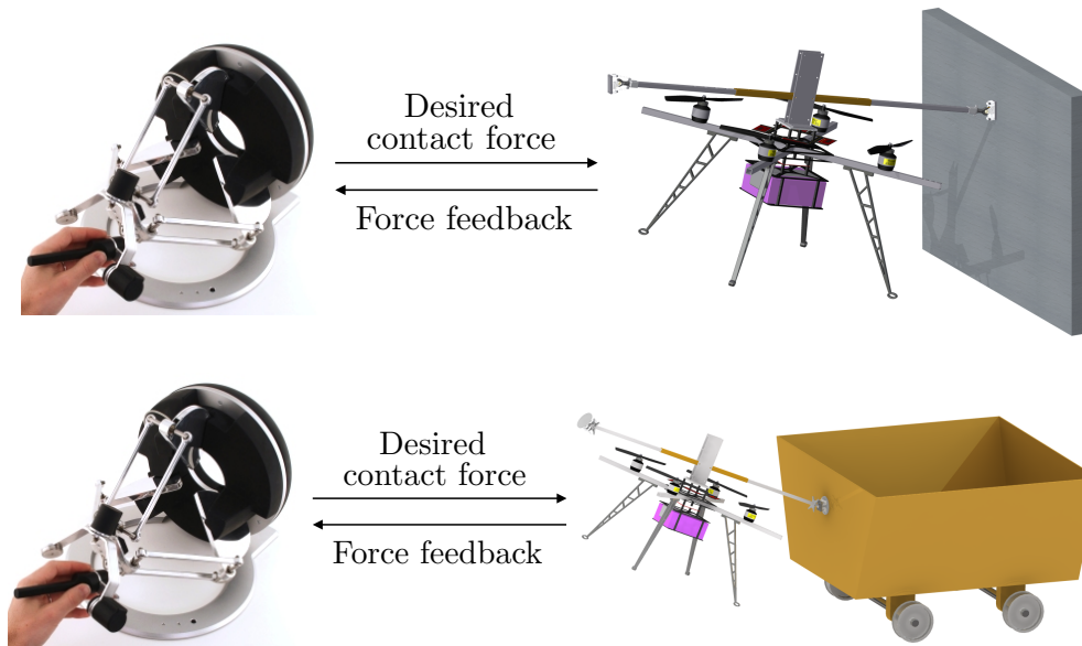
Figure 3.5: The scenarios of aerial teleoperation for physical interaction with contact considered in (Gioioso et al. 2015). Top: docking to a surface. Bottom: pushing a cart.
