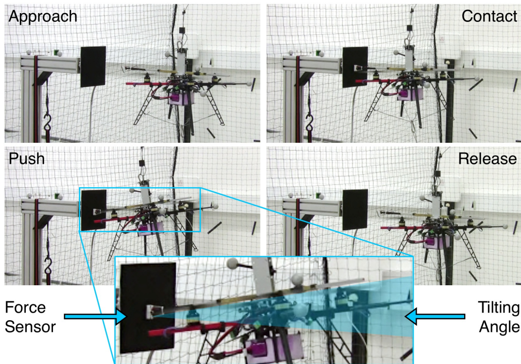
Figure 2.14: Experiments validating the controller of the force exerted by a quadrotor when using a rigid tool to physically interact with the environment.
