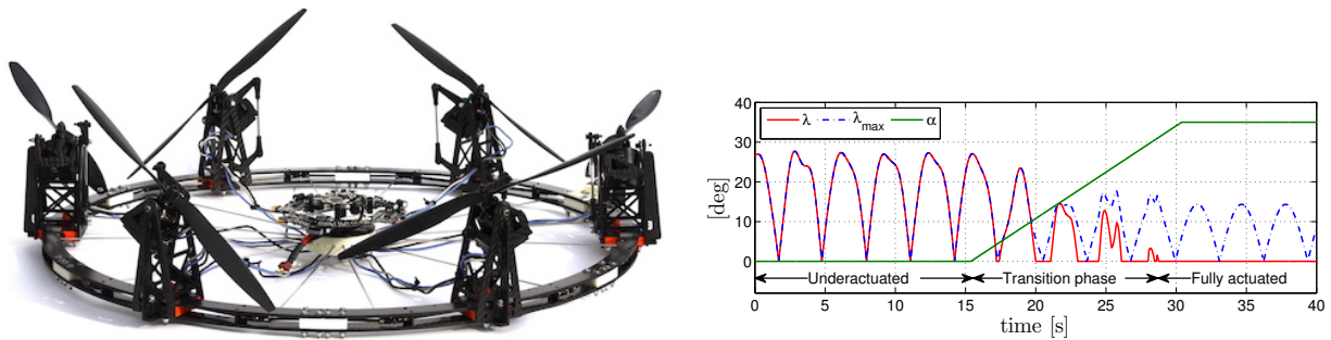
Figure 2.21: Left: one of the developed fully-actuated aerial prototypes. Right: smooth transition from under- to full-actuation.
