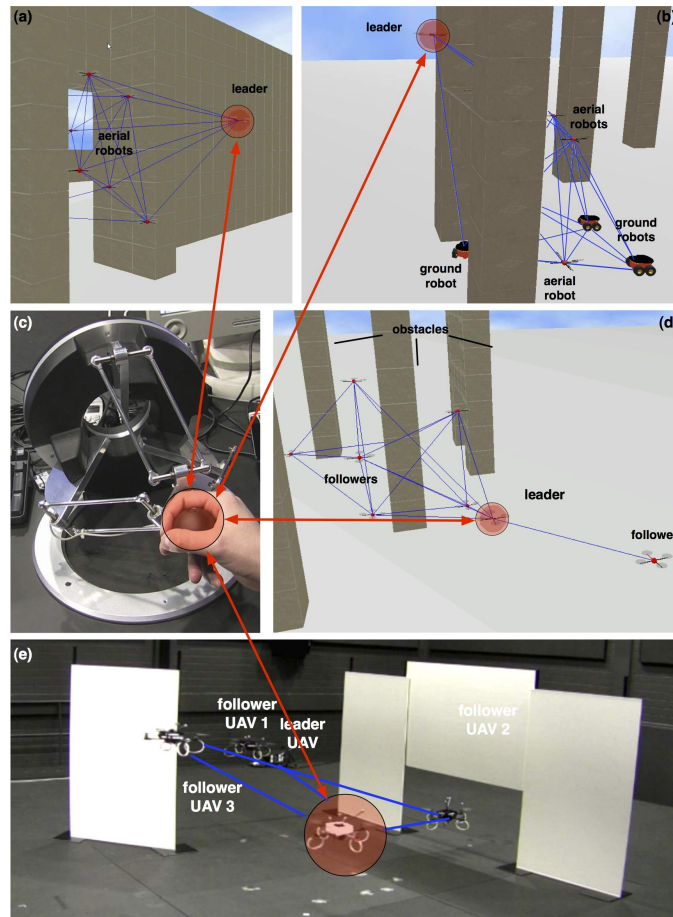
Figure 2.9: Simulations and experiments of shared control of multiple heterogeneous mobile robots.
