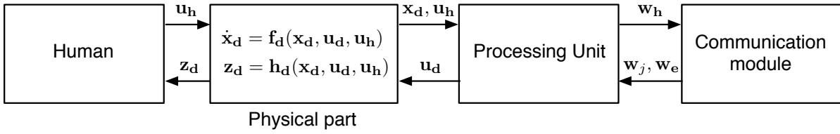
Figure 3.2: High-level model of the human-robot interface.
