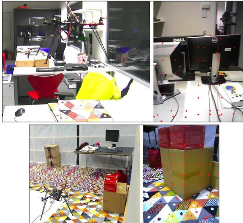
Figure 2.12: Semi-autonomous quadrotor that can be bilaterally teleoperated (i.e., with haptic feedback) by a remote user. The employed sensors are only the onboard RGB-D camera and IMU (no external motion capture is used).
