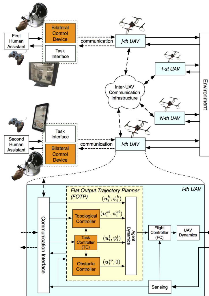
Figure 2.8: Architecture and overall framework of the shared control of multiple mobile robots.
