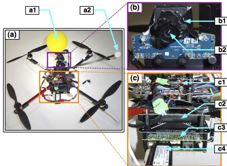
Figure 2.11: Quadrotor UAV developed for the experiments at MPI.
