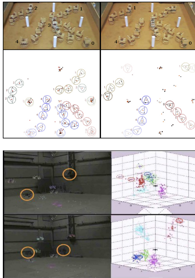
Figure 2.4: Experiments of the mutual localization method in the ground-robot and aerial-robot case.
