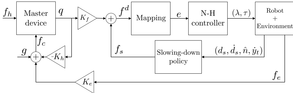
Figure 3.6: Block diagram of a control algorithm for aerial teleoperation in physical interaction with contact (Gioioso et al. 2015).
