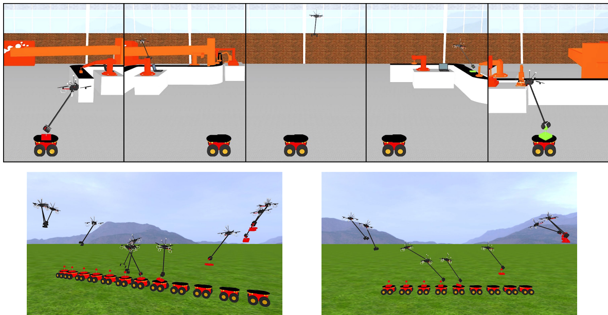
Figure 2.13: Dynamical simulations showing the planning strategy for allowing grasping of moving targets using an underactuated aerial robot equipped with a rigidly-attached gripper.
