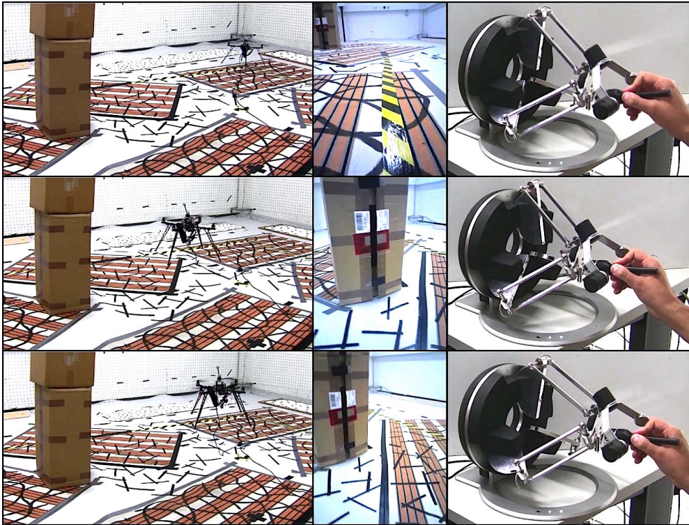
Figure 3.7: Experimental validation of a feedback-force collaboration scheme that uses onboard only sensors, namely an RGB-D camera and an IMU (Stegagno et al. 2014).
