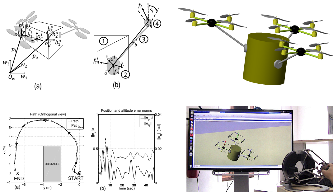
Figure 2.18: Human-in-the-loop simulations showing the developed cooperative aerial tele-manipulation control scheme. The robots perform a cooperative aerial grasping while taking into account all the main physical constraints of the system: joint limits, friction cones, maximum/minimum internal force, actuation limits, and smoothness of the control, to mention a few.
