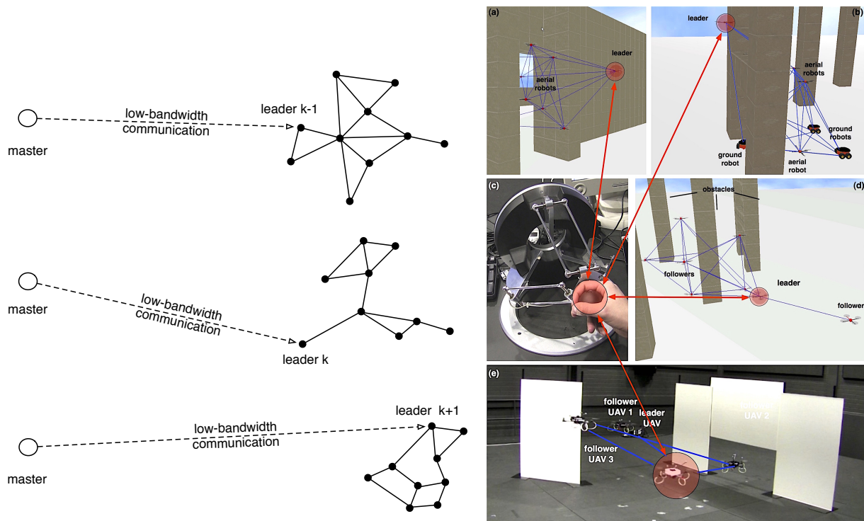
Figure 3.8: Left: abstraction of master-leader-followers scheme. The human operator (master agent) can communicate only with one robot at the time (the leader) using a low channel bandwidth. The leader robot and the followers communicated through a time-varying distributed communication topology.
