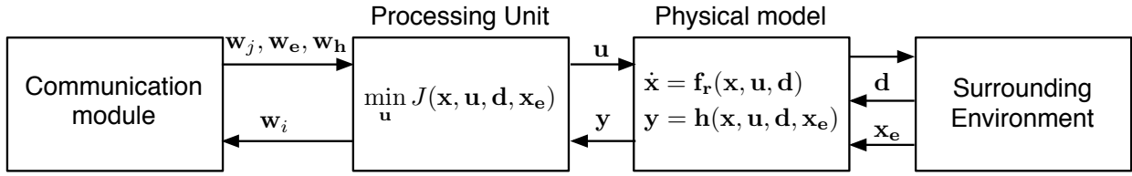
Figure 3.1: High-level model of the i -th mobile robot.
