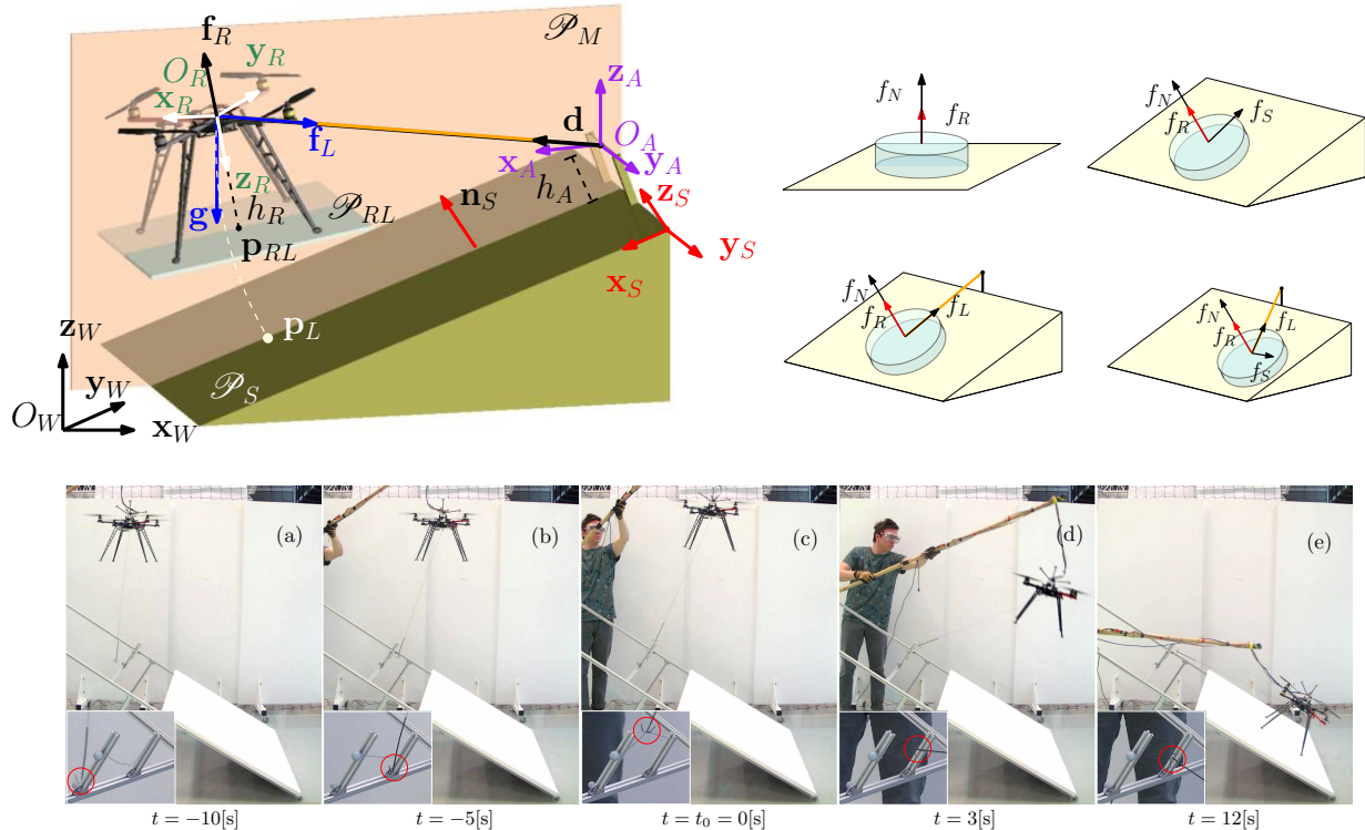
Figure 2.19: An experiment showing the use of the developed tethered control and planning methodology to robustly land on a sloped surface (perching).
