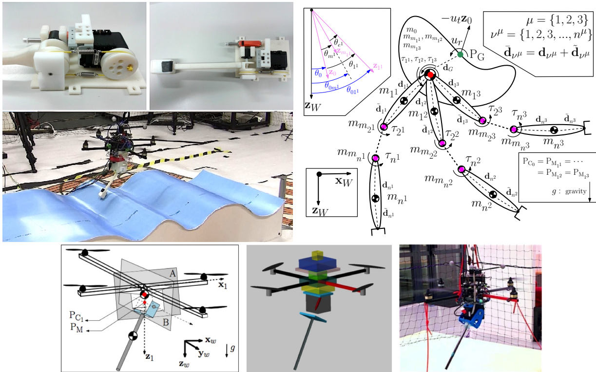
Figure 2.20: Experiments and kinematics of aerial manipulators with mixed rigid- elastic- joint arms. Top-left: a in-house developed elastic-joint arm for aerial manipulation. Bottom: a quadrotor equipped with a qbmove VSA elastic-joint from http://www.qbrobotics.com/ .
