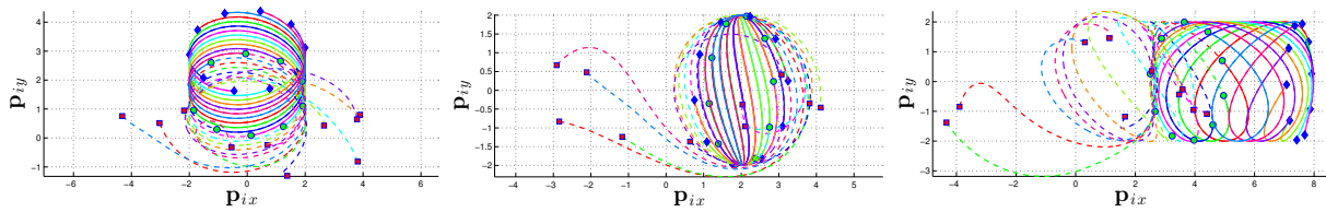
Figure 2.5: Examples of 3D trajectories generated by the decentralized encirclement control.
