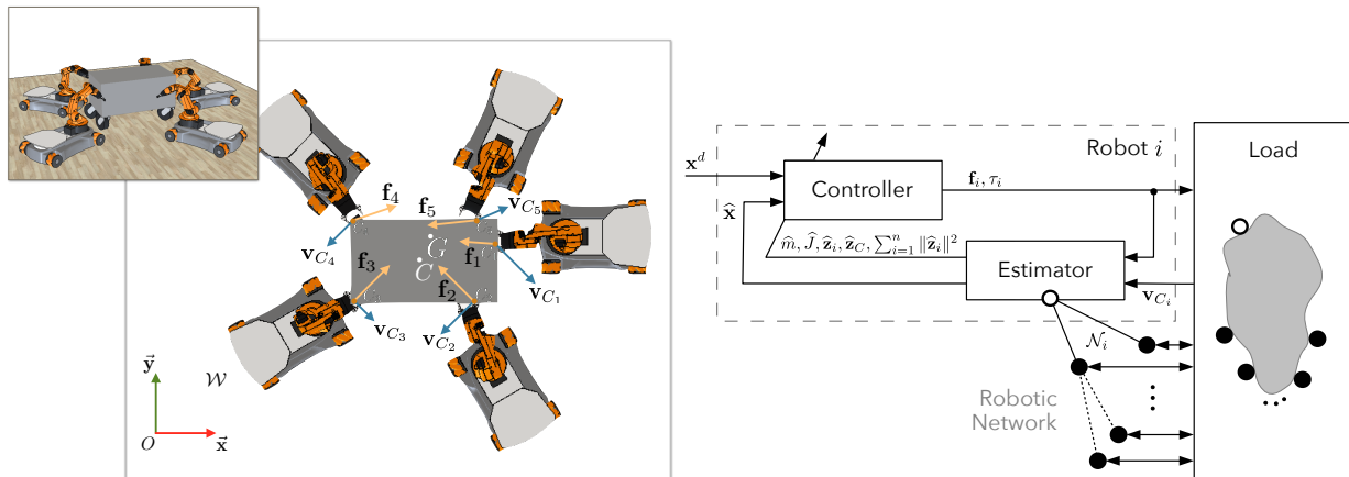
Figure 2.22: Fully-decentralized cooperative manipulation with unknown load parameters, unknown grasping parameters, and unknown load state.
