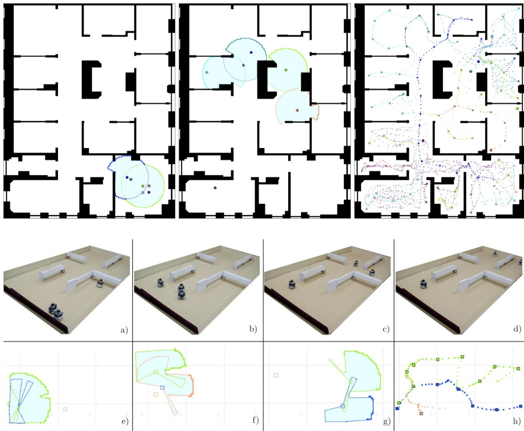
Figure 2.7: Simulations and experiments of the search without map method.
