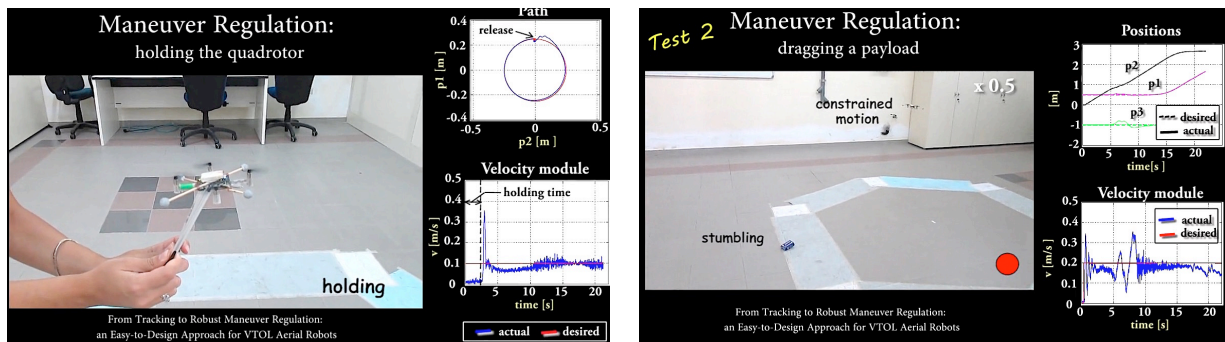
Figure 2.17: Experiments with a cm-scale aerial robot showing the robustness of the maneuver regulation approach (Spedicato, Franchi, and Notarstefano 2016) when the aerial robot is subject to unexpected external disturbances such as ‘holding’ (left) and ‘unknown payload dragging’ (right).
