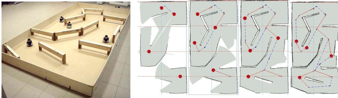
Figure 2.2: One of the experimental test of the SRG exploration method.
