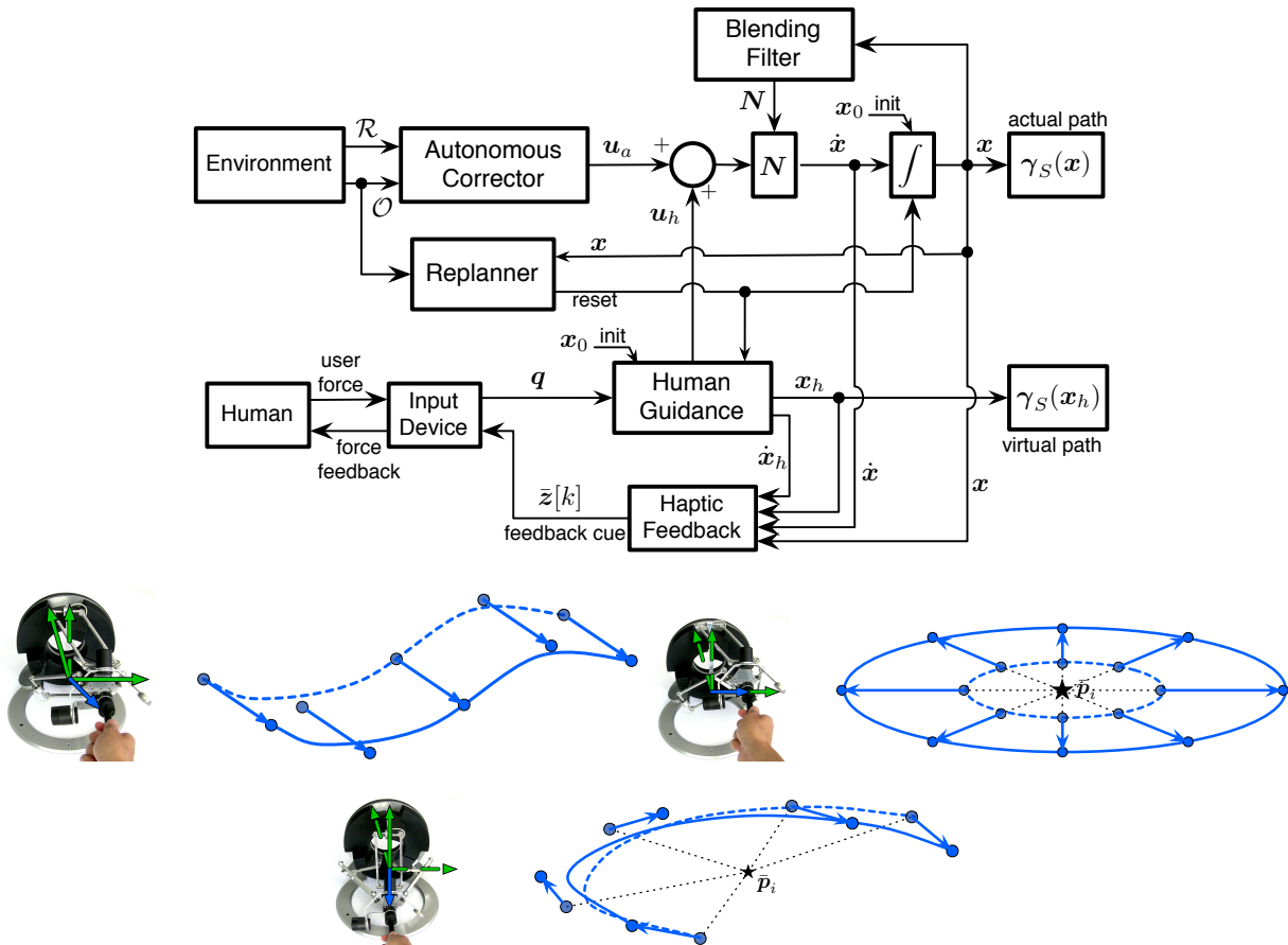
Figure 3.3: Top: block diagram of a feedback-force human-robot collaboration scheme with relatively long time horizon in the operator reference. Bottom: Examples of canonical path transformations. Green arrows represent the DoFs. Depending on the transformation the device motion is artificially restricted (continuous green arrows): 2 DoFs for translation, 1 DoFs for scaling, 1 DoFs for rotation. Blue arrows represent the commands and corresponding motion of the control points.
