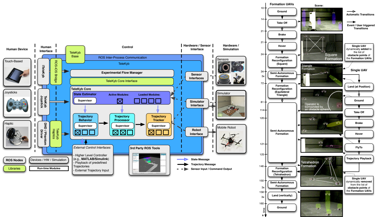
Figure 2.16: The TeleKyb software architecture allows a modular and extendible ROS-based control of single and multiple aerial robots with possible humans in the loop.
