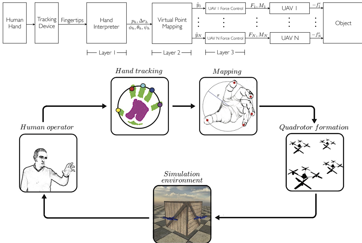
Figure 3.11: Block diagrams of the flying hand collaboration concept. Each aerial robot acts as a single finger to grasp an object and the is teleoperated by a human hand through the use of a suitable abstraction layer (Gioioso et al. 2014a).
