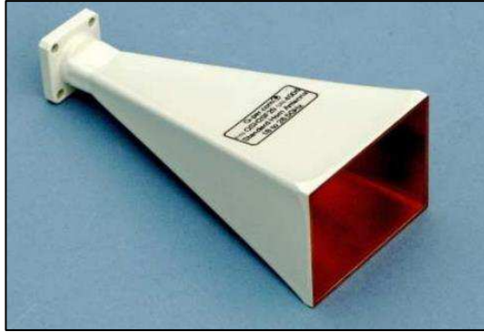
Figure 157. Antenne cornet (Q-PAR Antennas, Steatite)
