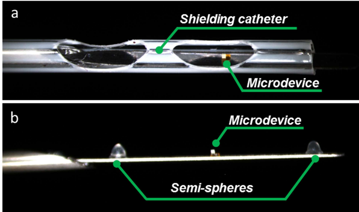
Figure 2.27 Proposed strategies to avoid the physical damage of the microdevice. a A customized catheter, containing two openings, shields the Nitinol strip. The microdevice and pillar are observed in one of the openings. b A couple of semi-spheres are fabricated at 3 mm from the microdevice, these are taller than the total height of the pillar and microdevice, thus prevent any direct mechanical contact on the microdevice.
