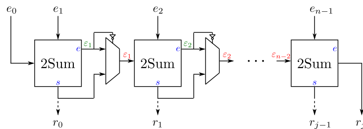
Figure 1.2 – Graphical representation of Algorithm 9. In the \text{2Sum} calls the sum s is outputted downwards and the error e to the right.
