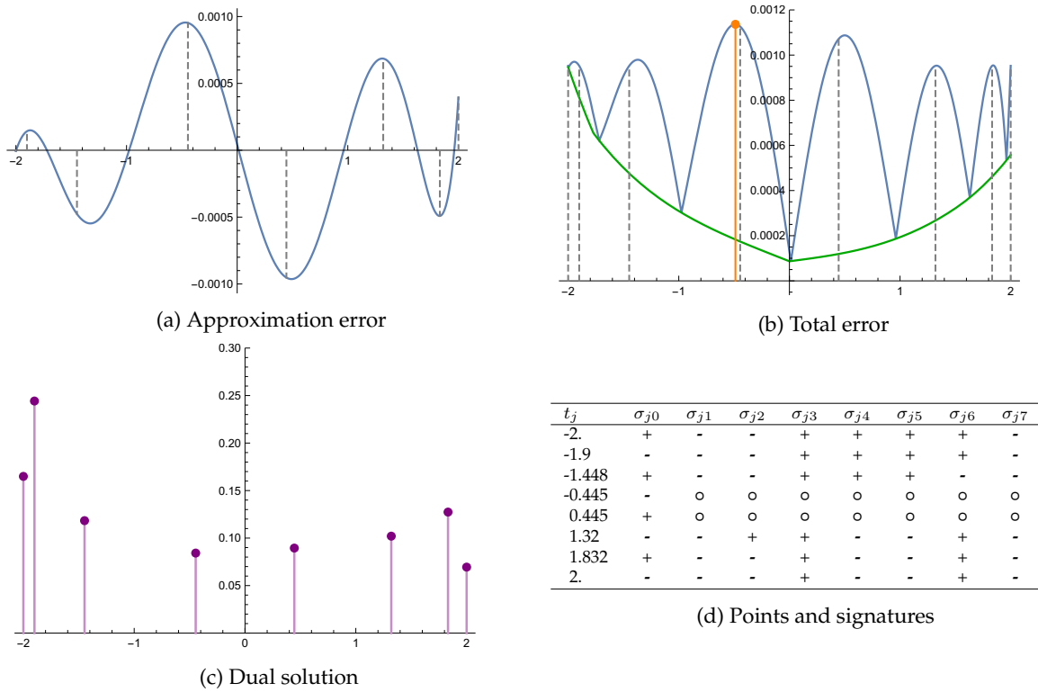
Figure 3.8 – Approximation of A_i over [-2, 2] : iteration 6
