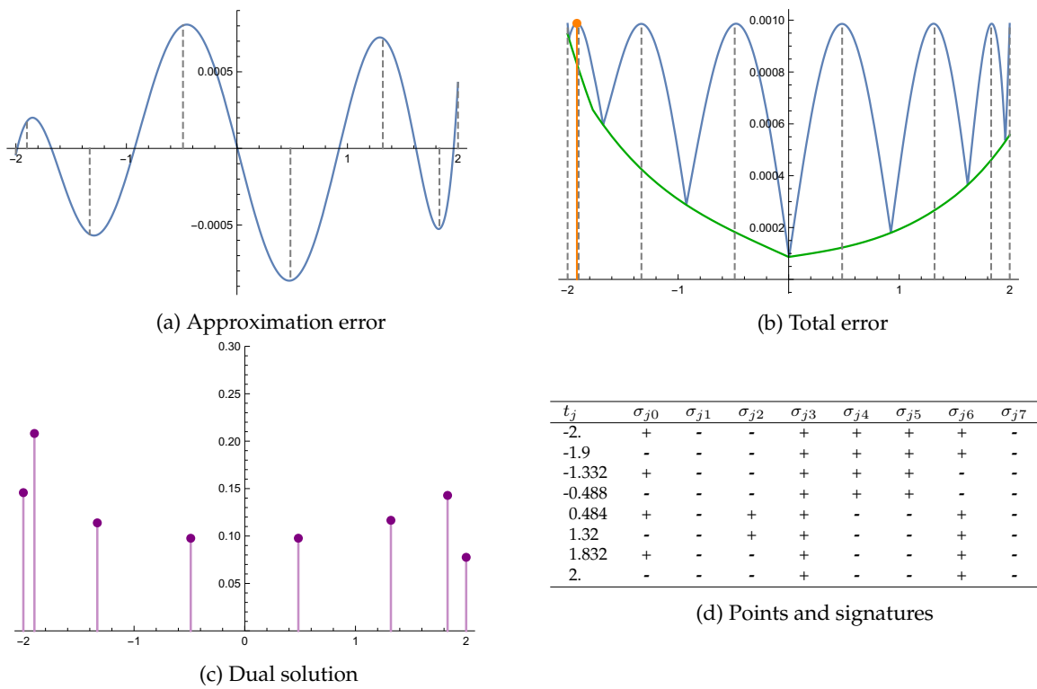
Figure 3.9 – Approximation of A_i over [-2, 2] : iteration 9
