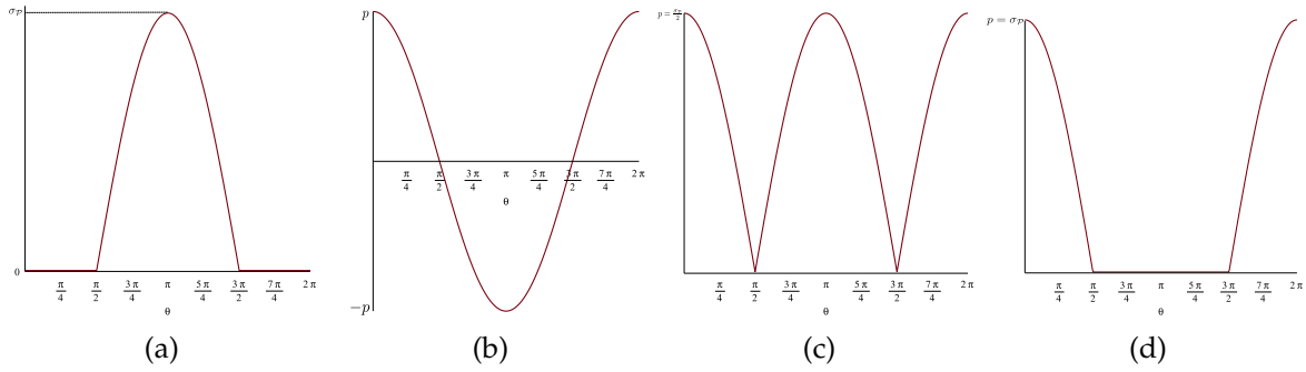
Figure 2.1 – Indicator functions of (a) probability g ; (b) precondition \xi \mapsto e^{p\xi} ; (c) \xi \mapsto e^{\frac{\sigma_g}{2}\xi}g(\xi) ; (d) \xi \mapsto e^{\sigma_g\xi}g(\xi) .
