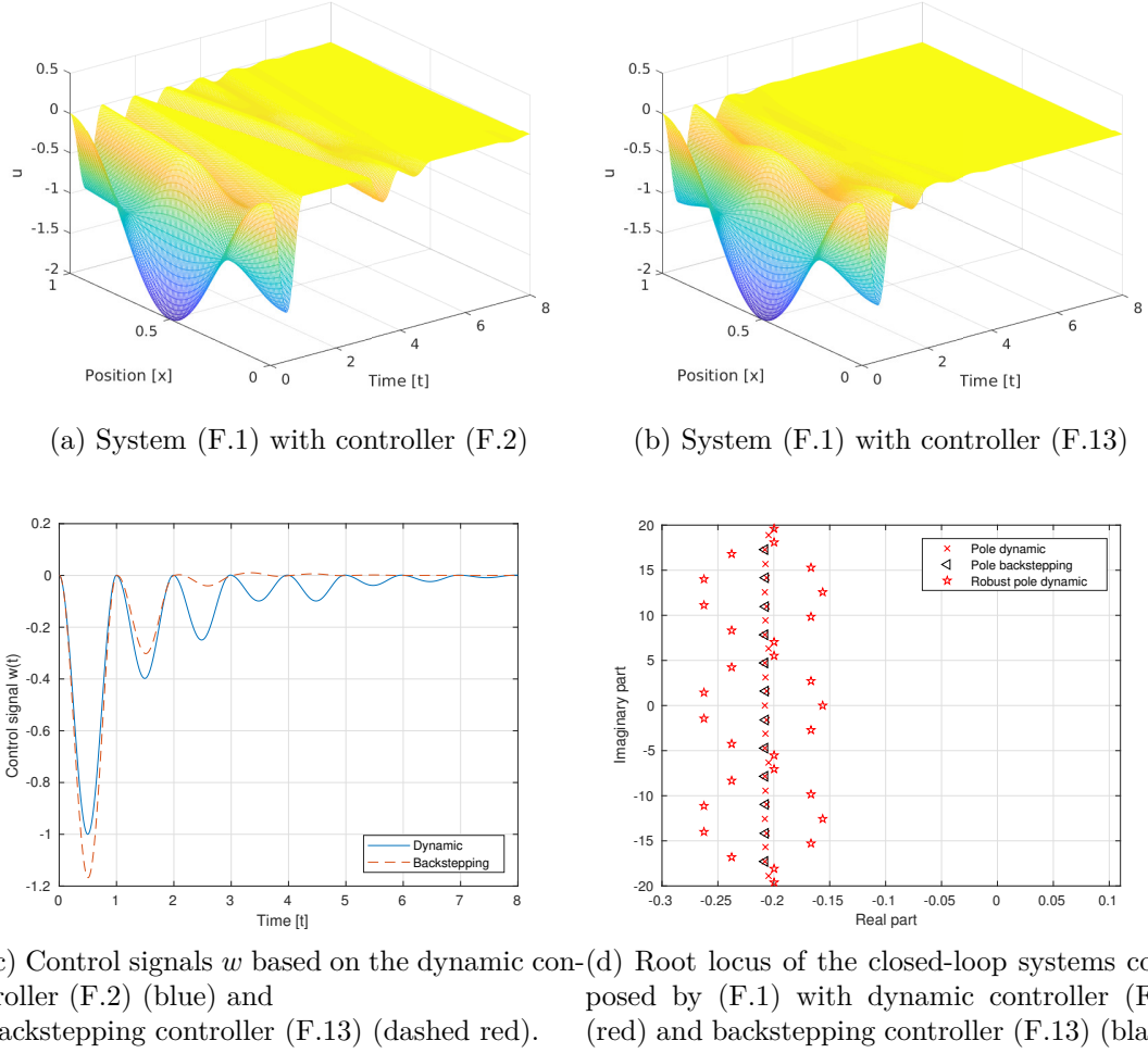
Figure F.4: System behavior depending on the controller. Figures (a) and (b) are simulations with initial conditions: u^0(x) = \cos(2\pi x) - 1 , u_t^0(x) = v^0(x) = v_t^0 = 0 for x \in (0, 1) . Figure (c) is a comparison between the two control laws. Figure (d) is a root locus comparison between the poles in three situations: backstepping (F.13) with parameters (F.14); dynamic controller (F.2) with parameters (F.14) and robust controller (F.2) with parameters (F.14) but a speed mismatch ( c_1 = 0.8 ).
