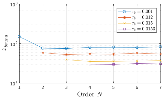
(a) k_p^\phi = 10^{-3} , k_i^\phi = 10 and \Omega_0 = 5 and some values of \tau_0 . The limit is z_{bound} = 29 .
