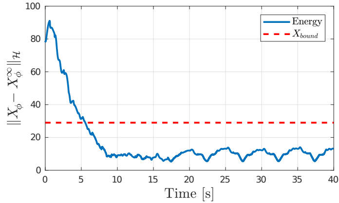
Figure 6.9: Energy of X_\phi for k_p^\phi = 10^{-3} , k_i^\phi = 10 and \Omega_0 = 5 . The initial condition is \phi^0(x) = (1 + 1.2 \sin(2x)) \int_0^x \phi_x^\infty(s) ds , \phi^1 = \Omega_0 and Z(0) = [z_1^\infty \ z_2^\infty]^\top .
