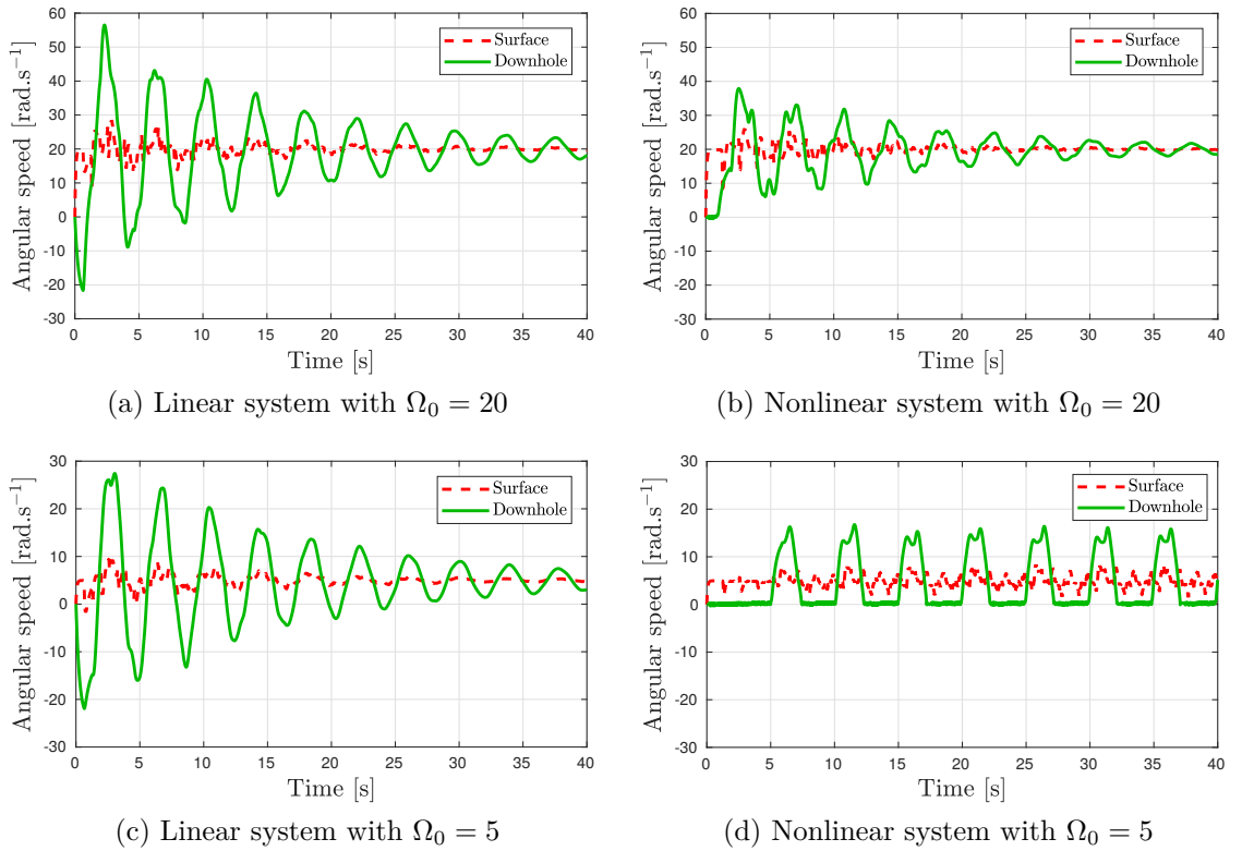
Figure 6.5: Numerical simulations for system (6.4) and (6.2) for two desired angular velocities and with a 0_{\mathcal{H}} initial condition.
