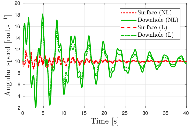
Figure 6.4: Numerical simulations for system (6.4) with k_p = 10^{-3} , k_i = 10 and \Omega_0 = 10 . The parameters are \phi^0(x) = (1 + 0.32 \sin(x)) \int_0^x \phi_x^\infty(s) ds , \phi^1 = \Omega_0 and Z(0) = (z_1^\infty \ z_2^\infty)^\top . (L) refers to the solution of the linear approximation and (NL) to the solution of system (6.2).
