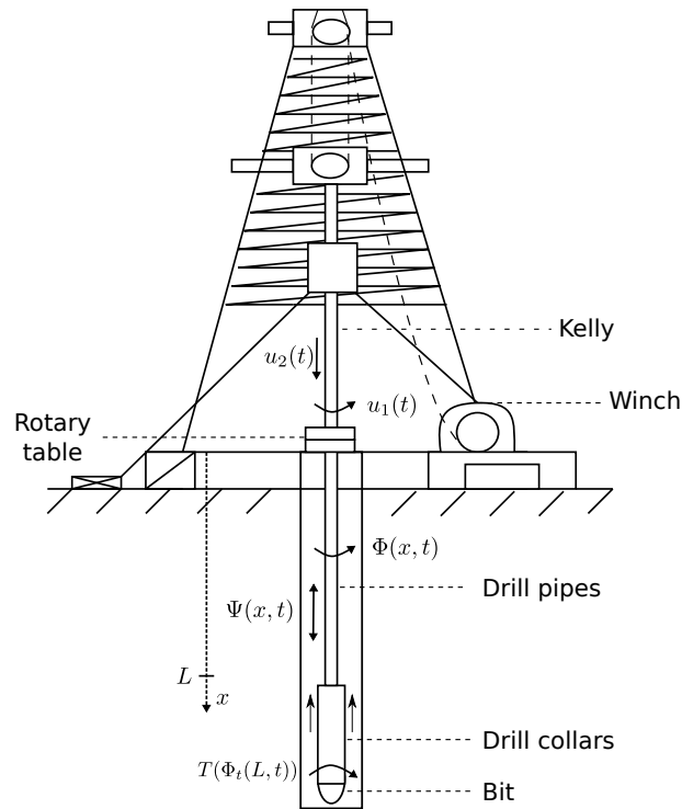
Figure 2.1: Schematic of a drilling mechanism originally taken from [136]. Data corresponding to physical values are given in Table 2.2.
