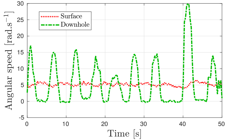
Figure 2.2: Nonlinear effect on the drilling mechanism due to the friction torque at the bottom of the pipe. These measurements are done on the field [142].
