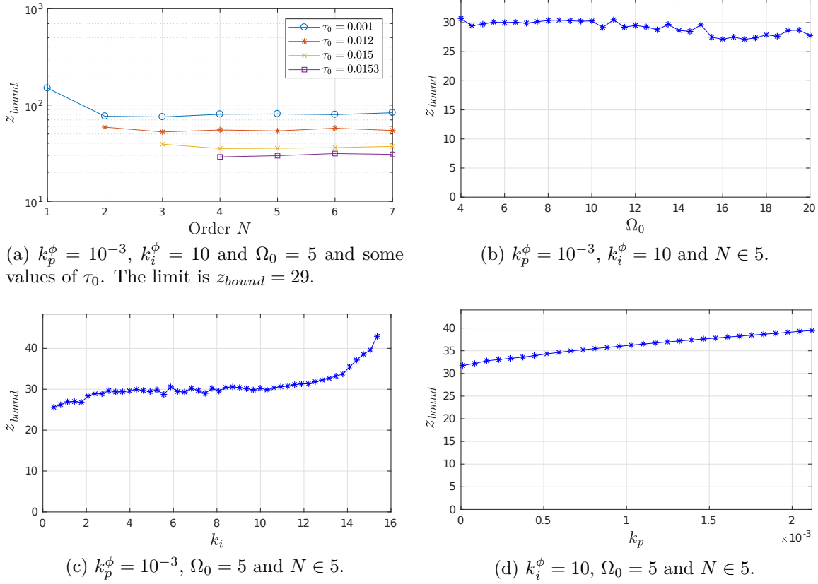
Figure 6.8: Solution z_{bound} of BMI (6.25) with algorithm 6.1.
