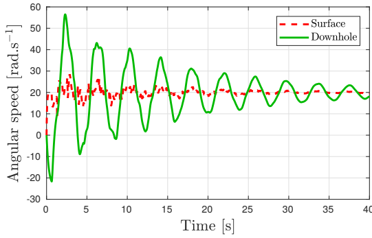
(a) Linear system with \Omega_0 = 20
