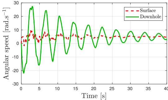
(c) Linear system with \Omega_0 = 5
