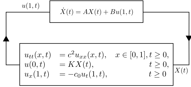
Figure 3.1: Block diagram for the system described by equation (3.1).
