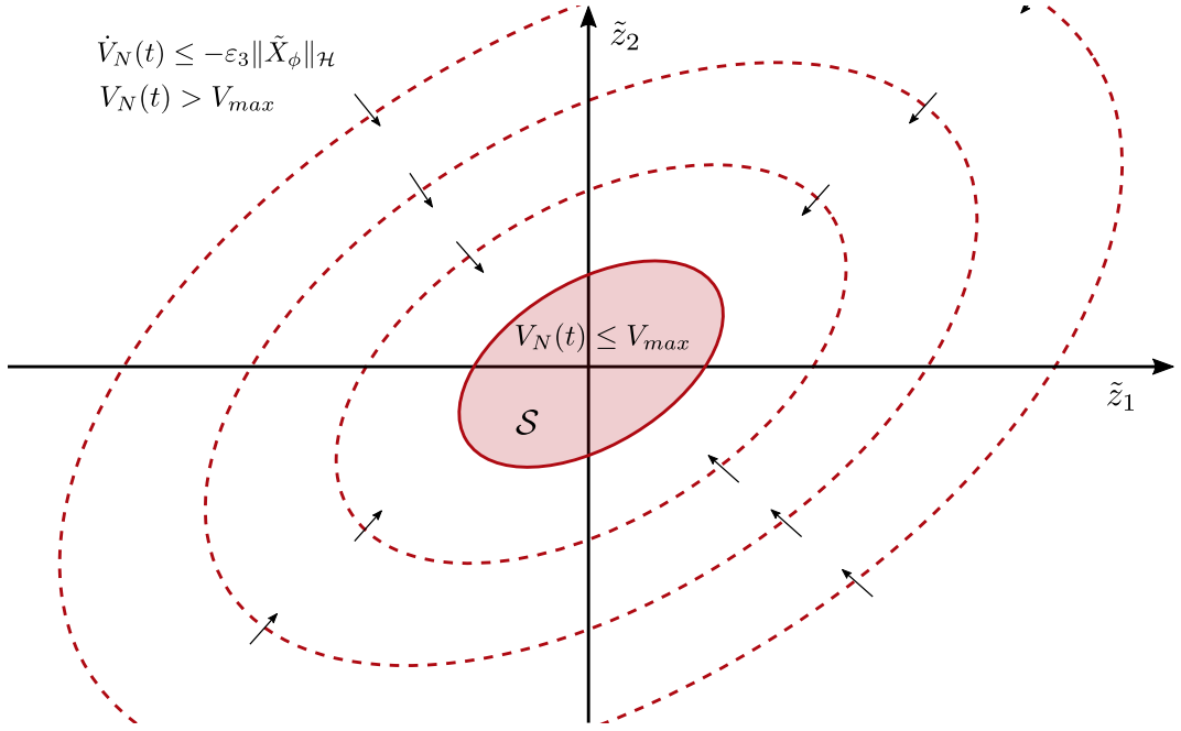
Figure 6.7: Illustration of the practical stability of (6.2). This is a projection of \tilde{X}_\phi on (\tilde{z}_1, \tilde{z}_2) . The dotted lines are isolines of V_N . The ball \mathcal{S} refers to V_N \leq V_{max} .
