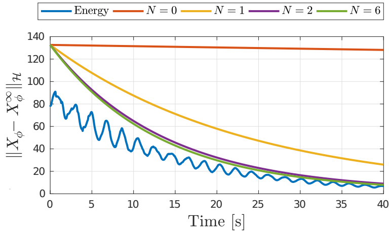
Figure 6.3: Energy of X_\phi with the linear system for k_p = 10^{-3} , k_i = 10 and \Omega_0 = 5 . The initial condition is \phi^0(x) = 4(\int_0^x \phi_x^\infty(s)ds + 0.1 \cos(2x)) , \phi^1 = 2\Omega_0 and Z(0) = 2[z_1^\infty \ z_2^\infty]^\top .
