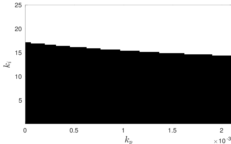
Figure 6.2: Values of gains k_p and k_i leading to a stable system with the maximum decay-rate for N = 5 using Theorem 1. The black area is stable and the white area is said unstable up to an order 5.
