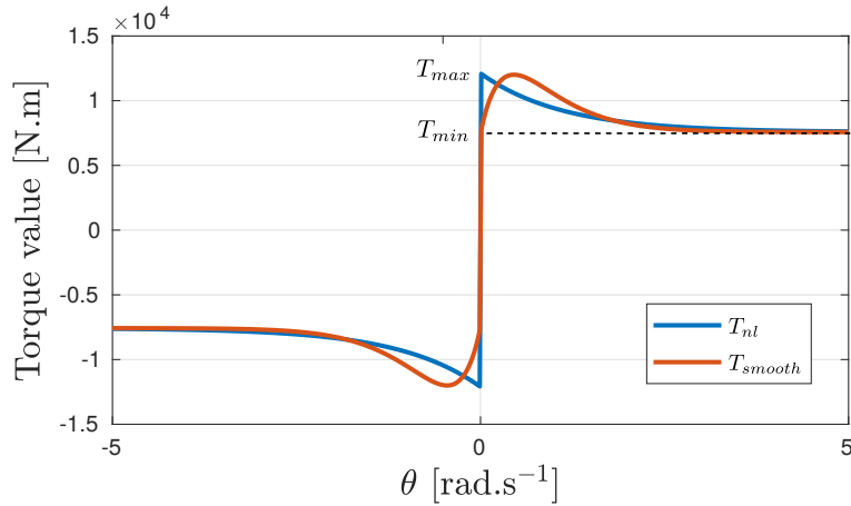
Figure 2.3: Nonlinear part of the torque. T_{nl} and T_{smooth} are both approximations of Karnopp's work [83] on friction.
