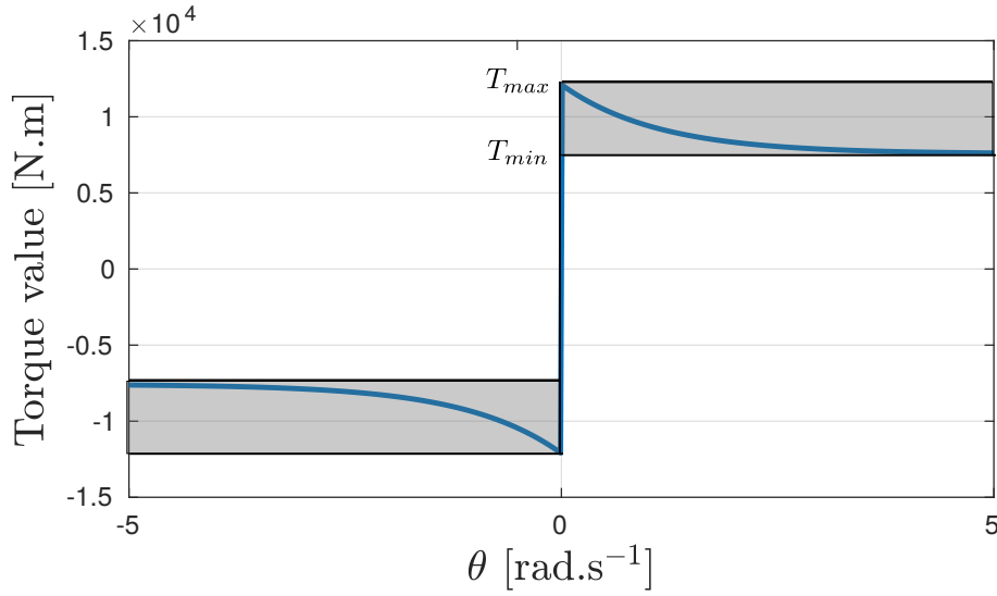
Figure 6.6: The sector conditions defined in (6.23) encapsulate the nonlinear T_{nl} inside the gray box.
