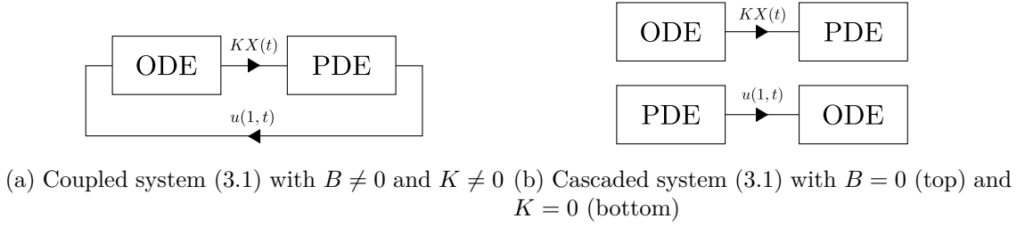
Figure 3.2: Block diagrams of coupled and cascaded systems represented by (3.1).
