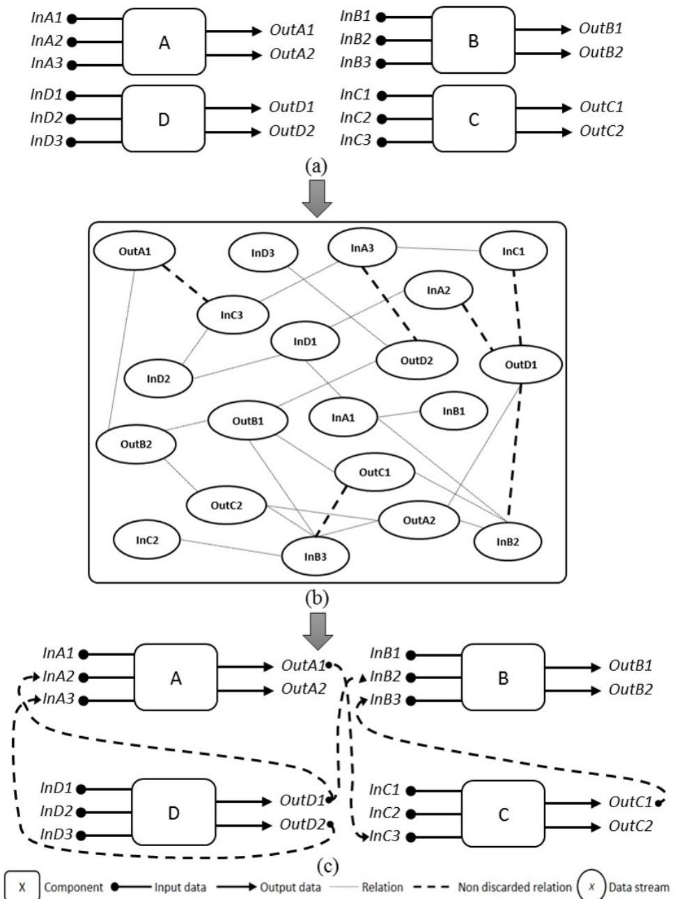
Figure 42: Example of Subsystem-to-Subsystem Graph Model building with DREAM
